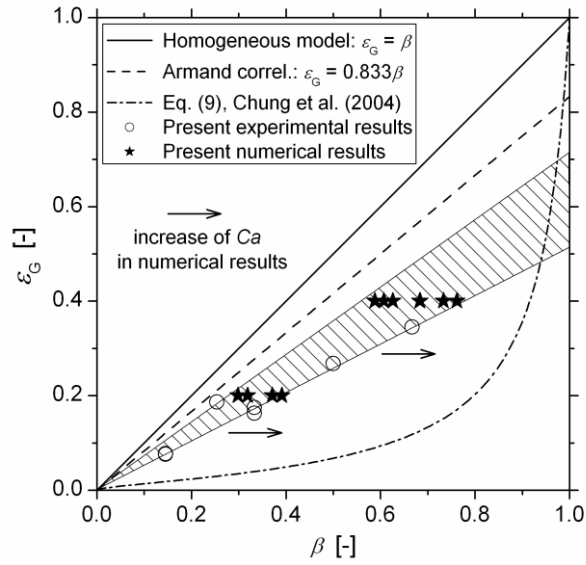
Figure 9. Gas holdup in the unit cell versus volumetric flow rate ratio. Comparison of the present experimental and numerical results with the homogeneous model, the Armand correlation 36 and Eq. (9) of Chung et al. 38 . The arrows indicate an increase of Ca in the simulations while the two lines enclosing the shaded area correspond to the fitting of the numerical data in Figure 8 by Eq. (7) and Eq. (8), respectively.
