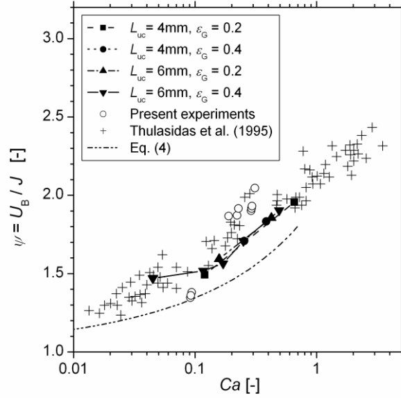
Figure 7. Ratio of bubble velocity to total superficial velocity versus capillary number.
