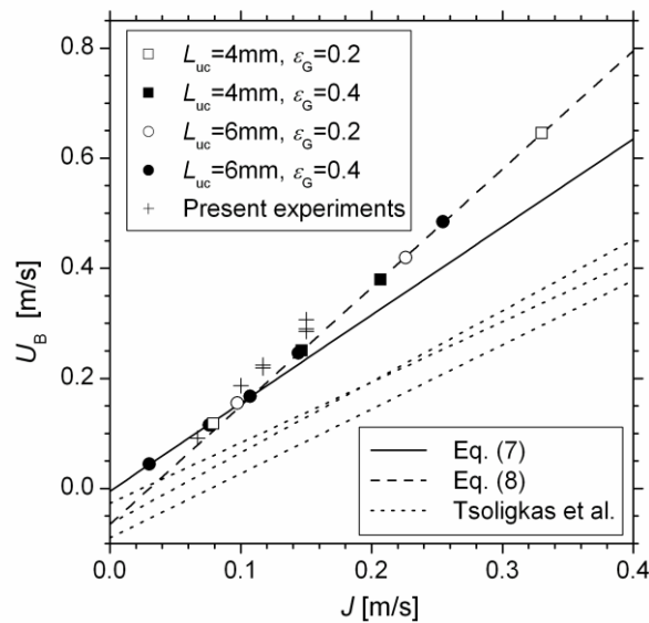
Figure 8. Comparison of present experimental (+) and numerical results (circles and squares) for bubble velocity versus total superficial velocity, and approximation of the numerical results by the drift-flux model, Eq. (7) and Eq. (8). The dotted lines correspond to the fitting of the experimental data of Tsoligkas et al. 15 by the drift-flux model.
