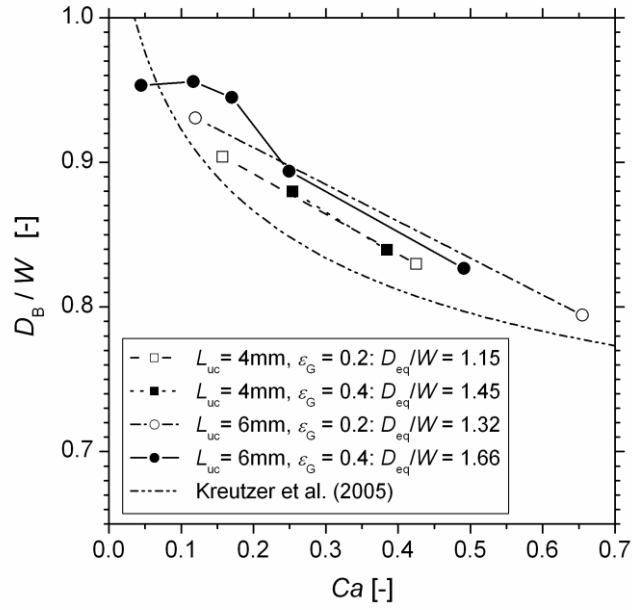
Figure 5. Bubble diameter versus capillary number. Comparison of simulation results with Eq. (1) from Kreutzer et al. 11 .
