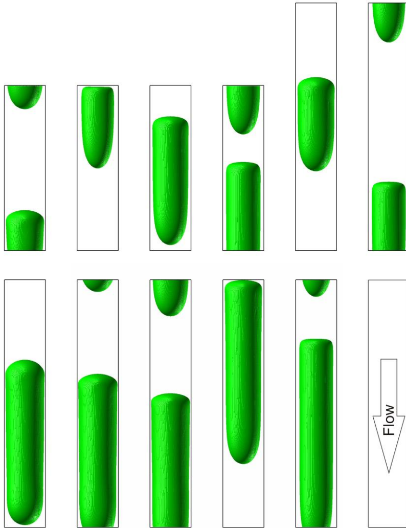
Figure 4. Lateral view of the three-dimensional bubble shape for all simulation runs. With reference to Table 1 the figure shows from left to right cases 4_20_A, 4_20_B, 4_40_A, 4_40_B, 6_20_A, 6_20_B (top row) and 6_40_A, 6_40_B, 6_40_C, 6_40_D, 6_40_E (bottom row).
