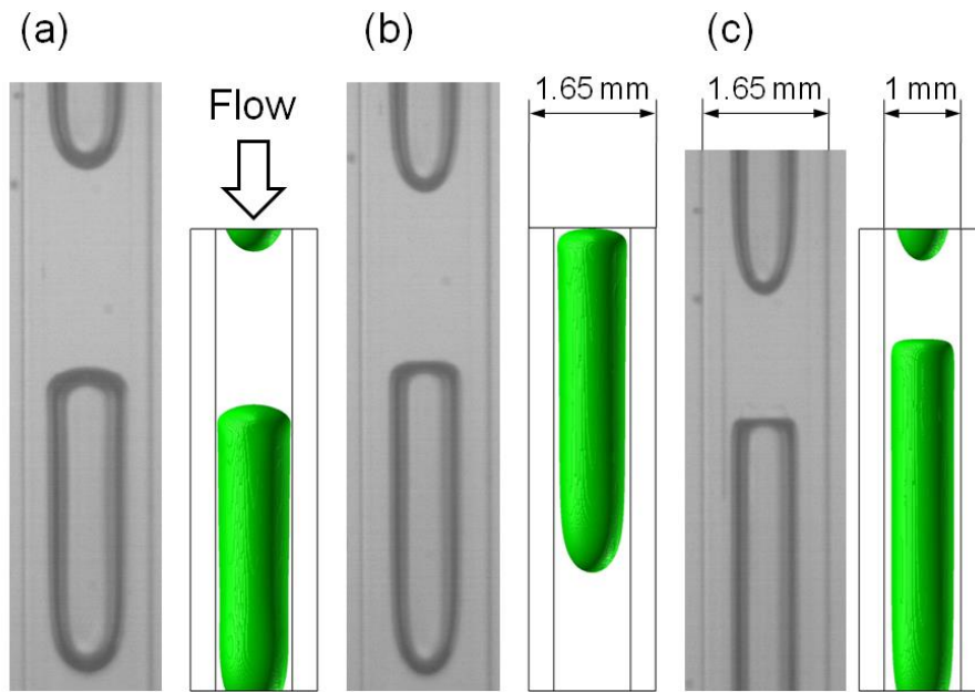
Figure 3. Comparison of bubble shape in experiment (left) and simulation (right) for similar liquid and gas superficial velocities. (a) (J_L, J_G)_{\text{Exp}} = (0.017 \text{ m/s}, 0.05 \text{ m/s}) , (J_L, J_G)_{\text{Sim}} = (0.03 \text{ m/s}, 0.046 \text{ m/s}) (case 6_40_B); (b) (J_L, J_G)_{\text{Exp}} = (0.05 \text{ m/s}, 0.1 \text{ m/s}) , (J_L, J_G)_{\text{Sim}} = (0.046 \text{ m/s}, 0.098 \text{ m/s}) (case 6_40_D); (c) (J_L, J_G)_{\text{Exp}} = (0.05 \text{ m/s}, 0.2 \text{ m/s}) , (J_L, J_G)_{\text{Sim}} = (0.061 \text{ m/s}, 0.194 \text{ m/s}) (case 6_40_E). For case denotations see Table 1.
