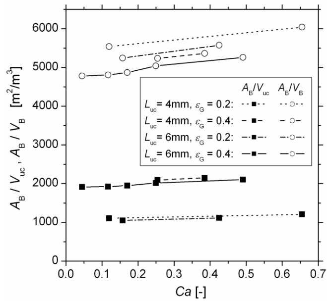
Figure 6. Simulation results for interfacial area per volume of the unit cell ( a_i=A_B/V_{uc} ) and interfacial area per bubble volume ( a_B=A_B/V_B ) as function of the capillary number.
