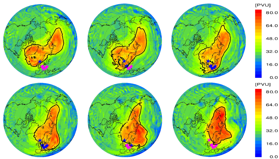
Fig. 6. Ertel's potential vorticity (PV; \times 10^{-6} \text{ K m}^2/\text{kg s} ) at \Theta=500 \text{ K} from 16 to 18 (top row) and 19 to 21 (bottom row) January 2006, from operational analyses of ECMWF for 12:00 UT; the boundary of the polar vortex (largest gradient of PV) is indicated by the thick black line; the six ozone sounding stations are marked by pink (outside vortex) and blue (inside vortex) stars.
