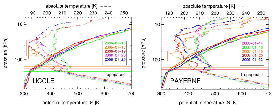
Fig. 4. Height profiles for Uccle (left panel) and Payerne (right panel) of potential temperature (lower x -axes, solid lines) and absolute temperature (upper x -axes, dotted lines), for same days as in Figs. 2 and 3; tropopauses were calculated following WMO criteria; vertical lines mark altitudes where the threshold for existence of PSCs of nitric acid trihydrate was reached.
