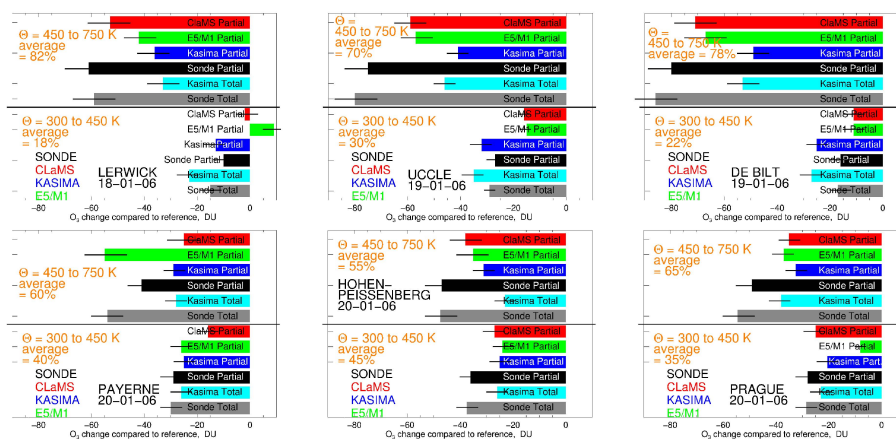
Fig. 15. Integrated ozone change between \Theta=300 and 450 K, and between \Theta=450 and 750 K at the six stations; sonde measurements in black and grey, KASIMA in blue and light blue, E5/M1 in green, CLaMS in red; Partial results for consistent common range ( \Theta=350 to 700 K); sonde and KASIMA also available for Total column between \Theta=300 and 750 K; average relative weights in % of the two altitude compartments to the total ozone decrease also given.
