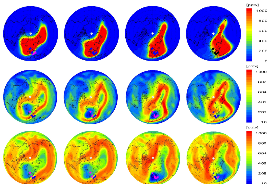
Fig. 13. Active Chlorine ( \text{ClO}_x , top row), chlorine nitrate ( \text{ClONO}_2 , middle row) and hydrochloric acid ( \text{HCl} , bottom row) as simulated by E5/M1 for 17 to 20 January 2006, 12:00 UT, for \Theta=500 K; the six sounding stations are marked by stars (different colours for better visibility).
