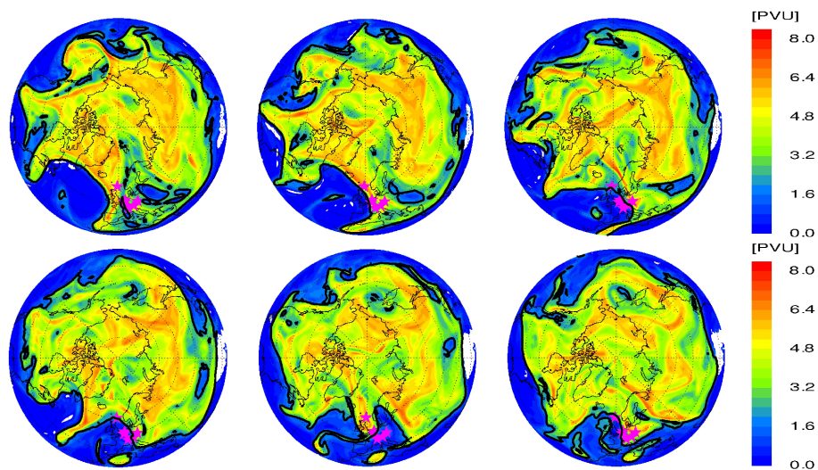
Fig. 5. Ertel's potential vorticity (PV; \times 10^{-6} \text{ K m}^2/\text{kg s} ) at \Theta=325 \text{ K} from 16 to 18 (top row) and 19 to 21 (bottom row) January 2006, from operational analyses of ECMWF for 12:00 UT; The six ozone sounding stations are marked by pink stars and the PVU=2 level by the thick black contour line.
