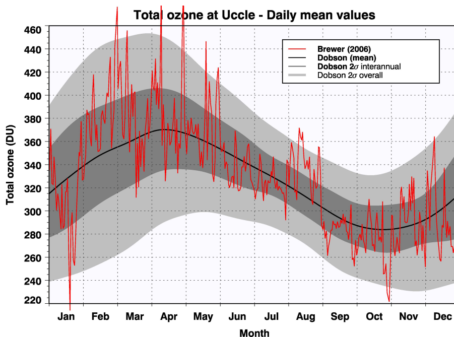
Fig. 1. Total ozone column measured at Uccle; the black line is the mean of all Dobson measurements since 1971, the light and dark grey-shaded area represent the 95%-percentile-bound (or 2\sigma error) of the overall and the interannual Dobson time-series variability, respectively (see also text). The daily averages of 2006 measured by Brewer No. 16 are given in red.
