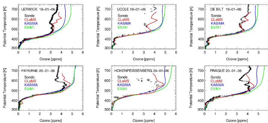
Fig. 11. Measured and simulated ozone profiles for the six ozone sounding stations, for the days when minimum total ozone was observed; ozone sonde data given by black crosses, CLaMS results by red, KASIMA results by blue, and E5/M1 results by green lines, respectively.
