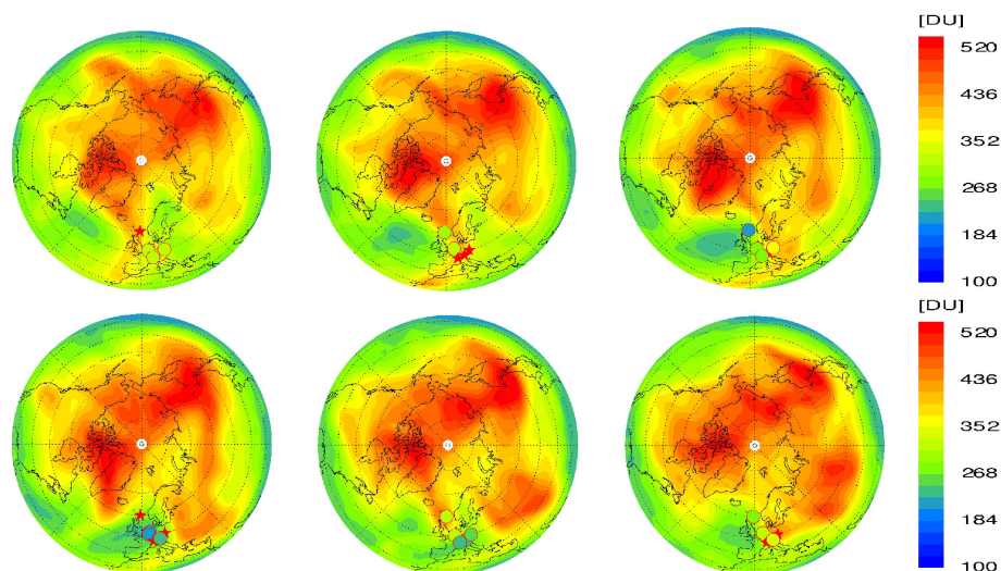
Fig. 9. Total ozone column in DU for 16 to 18 (top row) and 19 to 21 (bottom row) January 2006, 12:00 UT, simulated by E5/M1; sounding stations are marked either by red stars (no measurement) or by red circles (total column measurement available, circles filled in respective colour code for Dobson Units).
