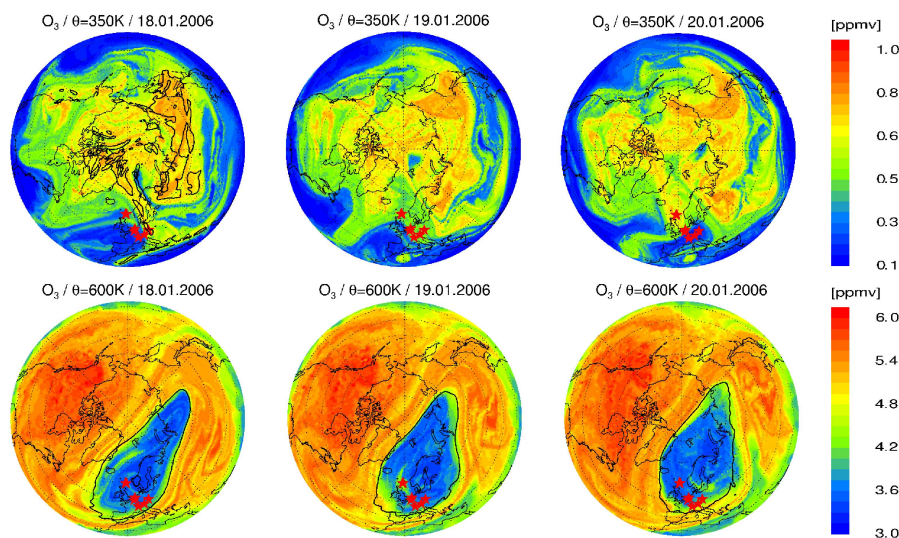
Fig. 10. Ozone mixing ratio in ppmv for 18, 19 and 20 January 2006, 12:00 UT, for \Theta=350 (top row) and \Theta=600 K (bottom row) as simulated by CLaMS; ozone sounding stations marked by stars; boundary of the polar vortex marked by the thick black line; note the different scales for \Theta=350 and 600 K.
