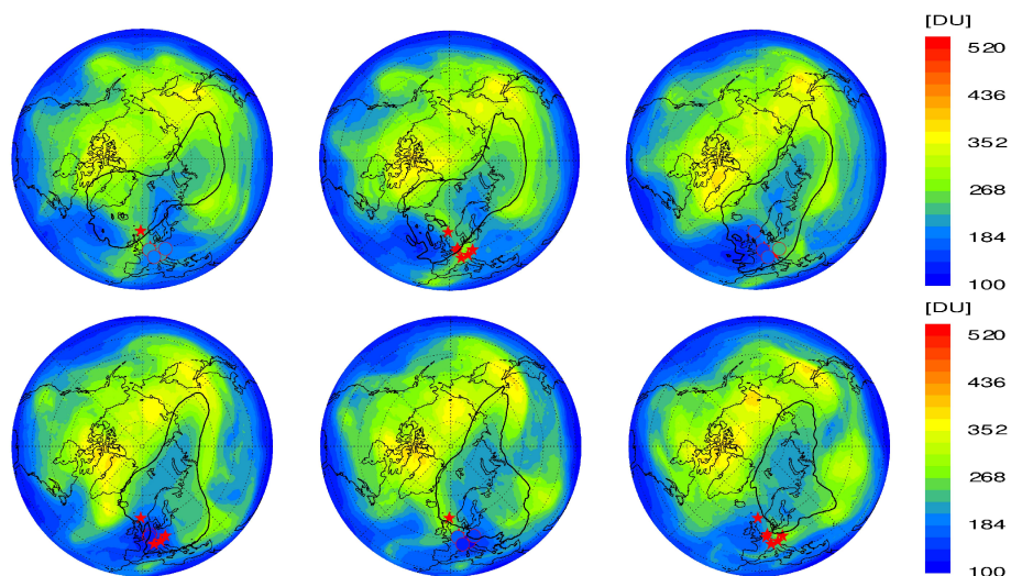
Fig. 7. Partial ozone column ( \Theta=350 to 700 K) in DU for 16 to 18 (top row) and 19 to 21 (bottom row) January 2006, 12:00 UT, simulated by CLaMS; boundary of the polar vortex is marked by the thick black line; sounding stations are marked either by red stars (no measurement) or by red circles (partial column measurement available, circles filled in respective colour code for Dobson Units).
