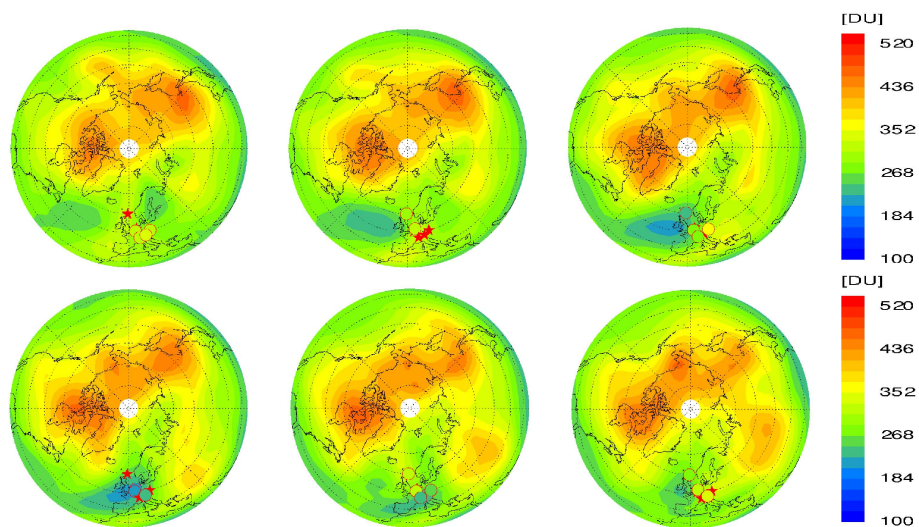
Fig. 8. Total ozone column in DU for 16 to 18 (top row) and 19 to 21 (bottom row) January 2006, 12:00 UT, simulated by KASIMA; sounding stations are marked either by red stars (no measurement) or by red circles (total column measurement available, circles filled in respective colour code for Dobson Units).
