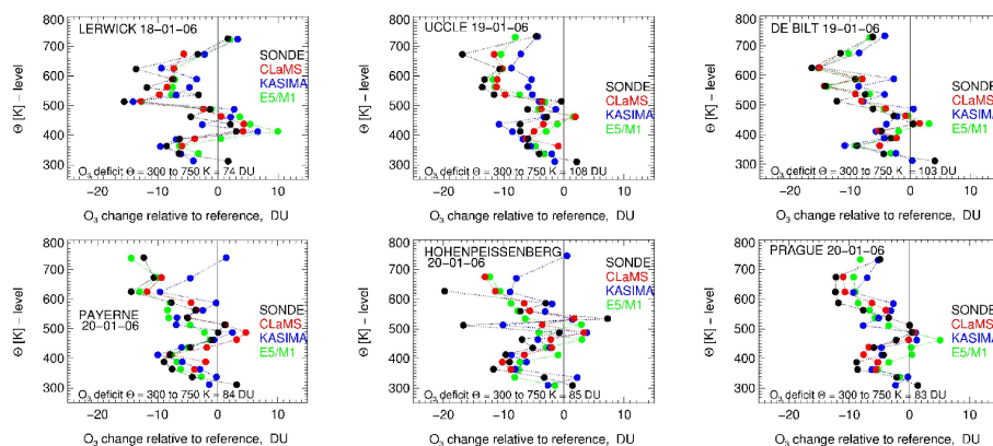
Fig. 14. Calculated ozone change in DU relative to the reference profiles, for observed (black points) and simulated (CLaMS=red, KASIMA=blue, E5/M1=green points) ozone profiles at the six stations and the days of observed minimum total ozone; dotted lines for guiding the eye; negative values correspond to lower (reduction), positive values to higher (gain) values than the reference; values integrated between certain Theta-level intervals (details see text).
