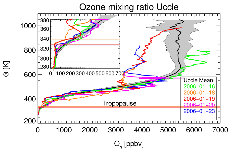
Fig. 2. Measured ozone profiles above Uccle in January 2006; the black line represents the mean of all Uccle soundings in January from 1995 to 2006 and the shaded area the 1\sigma standard deviation. Tropopauses were calculated following WMO criteria. The inserted image shows a zoom into the UTLS region, with ozone in ppbv against \Theta (K).
