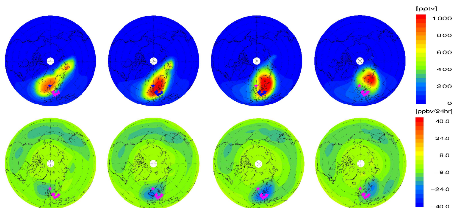
Fig. 12. \text{ClO}_x (top row) and over 24h cumulated chemical ozone change (bottom row) as simulated by KASIMA for 17 to 20 January 2006, 12:00 UT, for the 23.5 km height level (around \Theta=500 K); the six sounding stations are marked by stars (different colours for better visibility).
