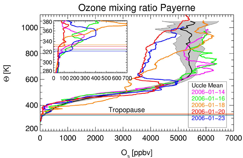
Fig. 3. Measured ozone profiles above Payerne in January 2006; the black line represents the mean of all Uccle soundings in January from 1995 to 2006 and the shaded area the 1\sigma standard deviation. Tropopauses were calculated following WMO criteria. The inserted image shows a zoom into the UTLS region, with ozone in ppbv against \Theta (K).
