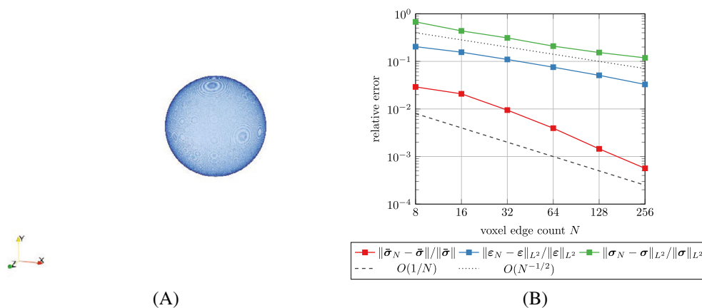
FIGURE 1 The single spherical inclusion. (A) Microstructure, (B) Convergence rates.
