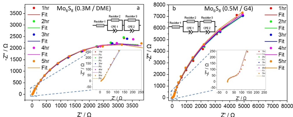
Figure 5. Nyquist plots of Mo 6 S 8 at SOC100%: a) in DME, b) in G4.
