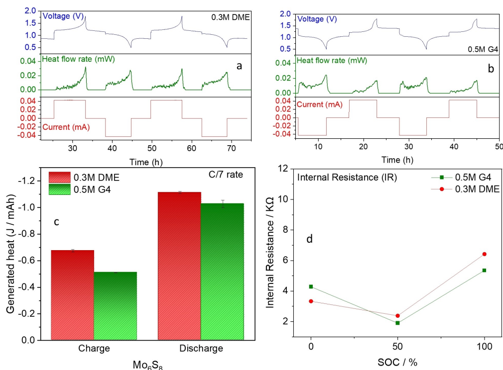
Figure 4. a) voltage, current and heat flow rate curves of Mo 6 S 8 in DME, b) voltage, current and heat flow rate curves of Mo 6 S 8 in G4, c) corresponding capacity-normalized generated heat for both systems for C/7 charge/discharge rate, d) dependence of internal resistance on SOC for Mo 6 S 8 in G4 and DME.
