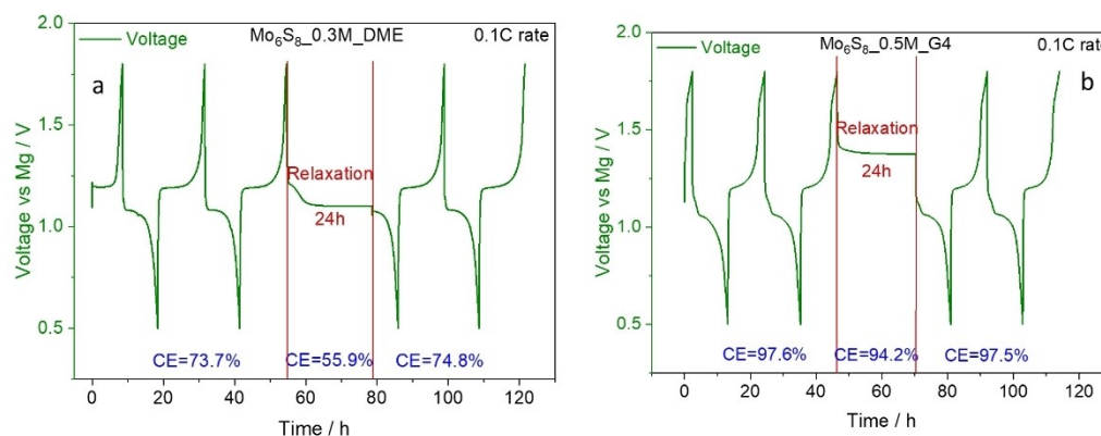
Figure 8. Self-discharge of a) Mo 6 S 8 in DME, b) Mo 6 S 8 in G4 with 0.1 C rate.
