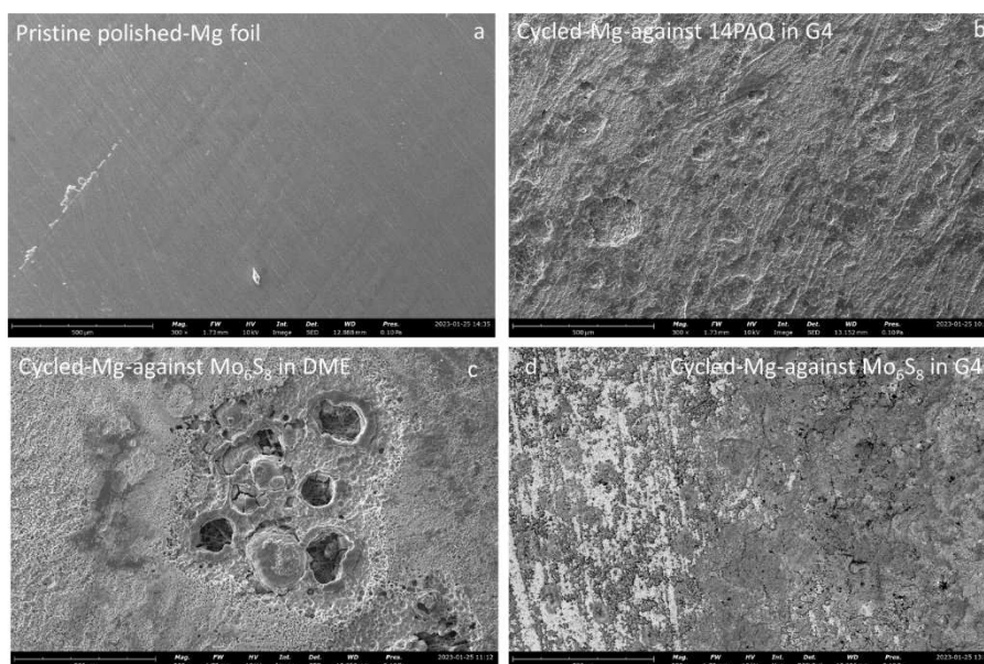
Figure 10. a) morphology of pristine polished-Mg anode, b) morphology of cycle-aged (200 cycles) Mg anode against 14PAQ in G4, c) morphology of cycle-aged (200 cycles) Mg anode against Mo_6S_8 in DME, d) morphology of cycle-aged (200 cycles) Mg anode against Mo_6S_8 in G4. The scale bars are 500 \mu m .
