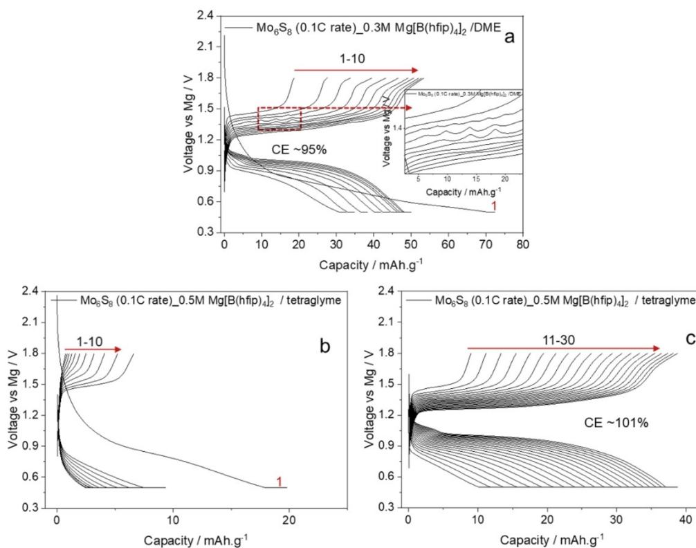
Figure 1. Comparison of the voltage vs. capacity curves during formation/activation of coin cells: a) first 10 cycles for Mo 6 S 8 in DME solvent, b) first 10 cycles for Mo 6 S 8 in G4 solvent, c) additional 20 cycles for Mo 6 S 8 in G4 solvent.
