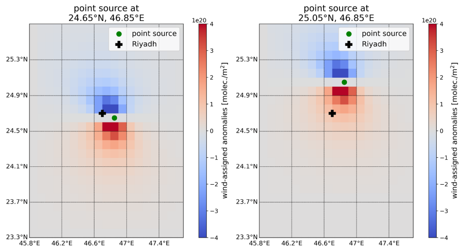
Figure A3. Examples of a wind-assigned plume for the point sources at 24.65° N, 46.85° E and at 25.05° N, 46.85° E in Riyadh.
