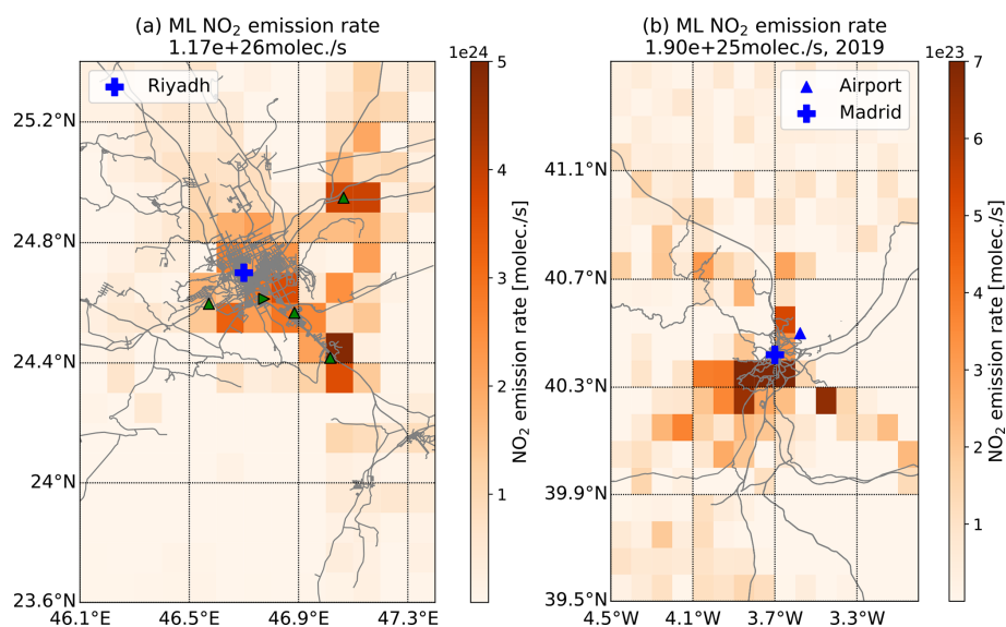
Figure 8. Panel (a) is similar to Fig. 1d but using southwest–northeast wind field segmentation; panel (b) is similar to Fig. 2d but using southeast–northwest wind field segmentation. Note that data are based on TROPOMI data in 2019.
