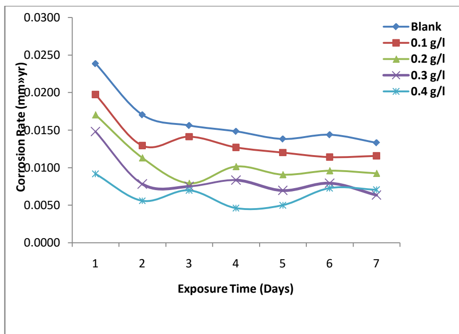
Fig.4: Corrosion Rate against Exposure Time of Al alloy in different concentrations of Mangifera indica leaf extract in 0.8 M HNO 3
