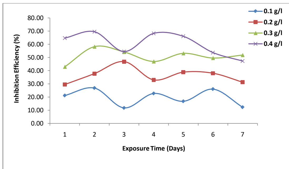
Fig.6: Inhibition Efficiency of Different Concentrations of Mangifera indica leaf Extract on Al alloy in 0.8 M HNO 3
