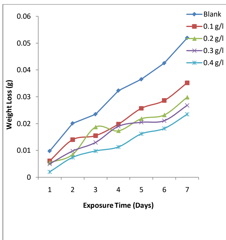
Fig.1: Weight Loss against Exposure Time of Al alloy in different concentrations of Mangifera indica leaf extract in 0.3 M HNO 3
