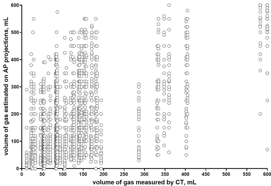
FIGURE 2 Abdominal gas volume. Relation between objective gas volumes measured by CT and estimated volumes on plain AP projections. Individual data of 48 observers for 60 images are shown. Note, great overlap of estimated values, even with largest gas volumes
