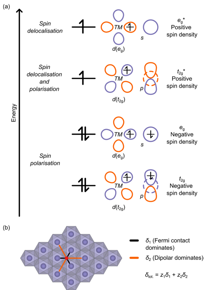
Figure 2. Illustrations of the hyperfine interaction in NMR. (a) The Fermi contact (through-bond) interaction of unpaired electron density on TM cations with a neighboring O nucleus. The bonding ( t_{2g} and e_g ) and anti-bonding ( t_{2g}^* and e_g^* ) combinations of TMd orbitals and s or p orbitals on O result in different spin density transfer processes. Bonding combinations cause spin polarization of electrons in filled s orbitals on O, while anti-bonding combinations cause spin delocalization (and polarization, in the case of the t_{2g}^* interaction). The sign of the spin density induced at the s orbitals (which defines the Fermi contact shift) is indicated to the right. (b) The interaction of the O nucleus with the nearest-neighbor and next-nearest-neighbor unpaired electron spins in the TMO 2 layer (of which there are z_1 and z_2 ) of a typical layered LIB cathode. These paths induce hyperfine shifts of \delta_1 and \delta_2 , respectively, giving a total shift of \delta_{\text{tot}} .
