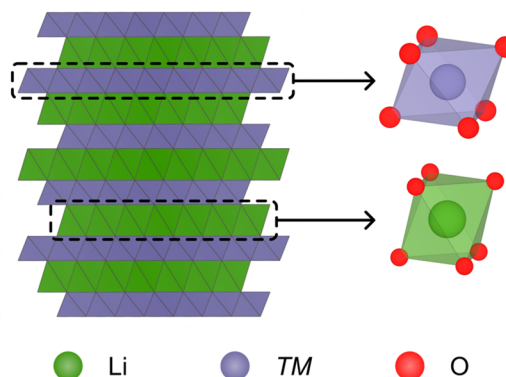
Figure 1. Crystal structure of a layered LIB cathode, \text{LiTMO}_2 , with the layers and local TM and \text{Li}^+ coordination polyhedra highlighted.
