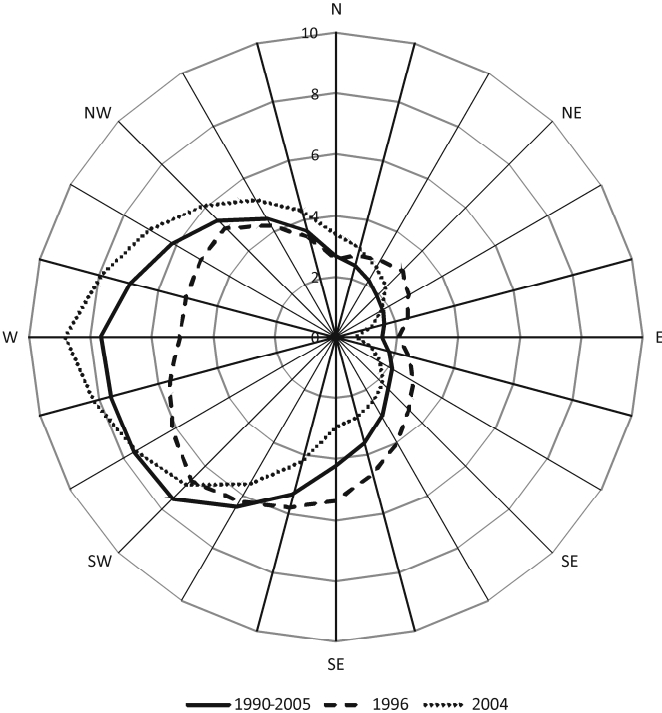
Fig. 1. The 1990-2005 average wind frequency rose compared to 1996 and 2004 wind frequency roses. Radial units are percent per 15° direction band (%)
