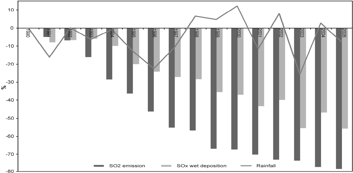
Fig. 5. Percentage change in average network precipitation, national SO 2 emissions and SO x wet deposition normalised against 1990 baseline
