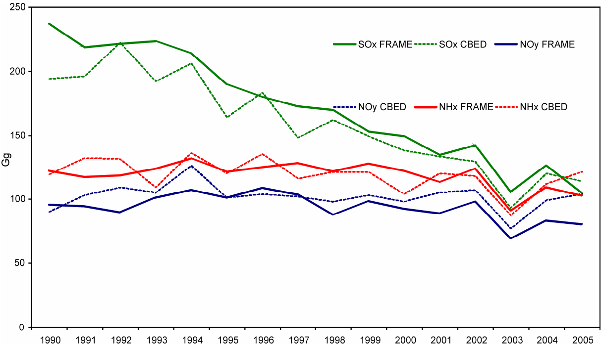
Fig. 3. Modelled and measured UK national wet deposition budget for: S-SO x , N-NO y , N-NH x (Gg)
