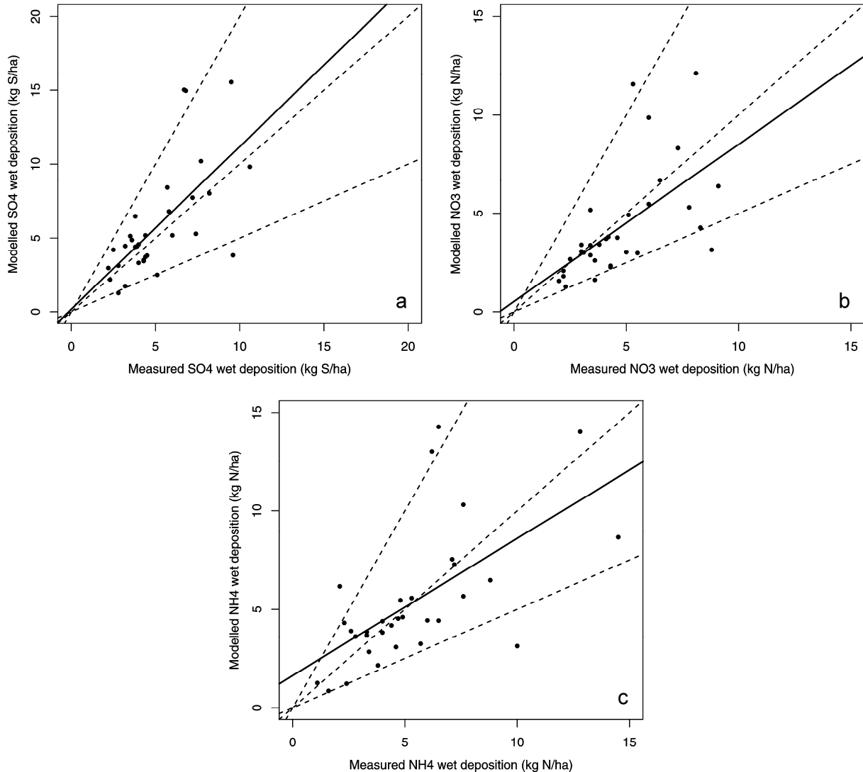
Fig. 2. Correlation of modelled wet deposition with measurements from the national monitoring network for 2005: a) SO 4 2- , b) NO 3 - , c) NH 4 + . Solid line is the best fit line produced by a regression analysis, dashed lines are for reference: 2:1, 1:2 and 1:1 division
