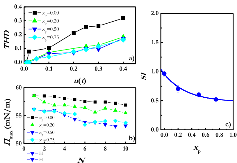
Figure 5. (a) Dependence of the total harmonic distortion calculated from the data in the FFT spectra using eq 3 on the deformation amplitude for a monolayer of LS with the incorporation of different particle mass fractions. (b) Dependence of the \Pi_{\max} on the number of compression–expansion cycles for LS films upon the incorporation of different particle mass fractions. (c) Dependence of SI on the particle mass fraction incorporated into the LS film. The data correspond to the average over 10 compression–expansion cycles, and the error bars represent the standard deviation. Data in all panels correspond to experiments around a reference surface pressure in the range 35–45 mN/m and deformations with u = 0.40 and \nu = 0.05 Hz, which are typical conditions that allow mimicking the respiratory cycle. In all of the panels, the lines are guides for the eyes.
