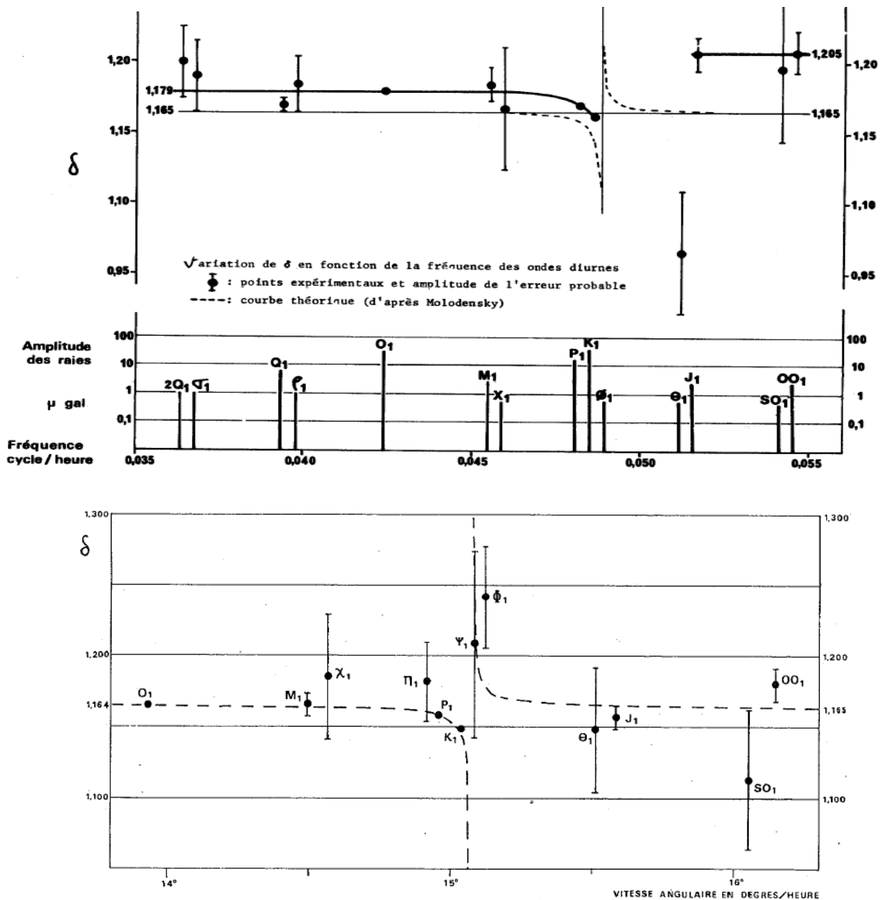
Fig. 6.7: Diurnal tides amplitude factors obtained by Lecolazet and Steinmetz in 1973 (up) and in 1974 (down) illustrating the improvement in \text{PSI1} amplitude determination between these two studies.
