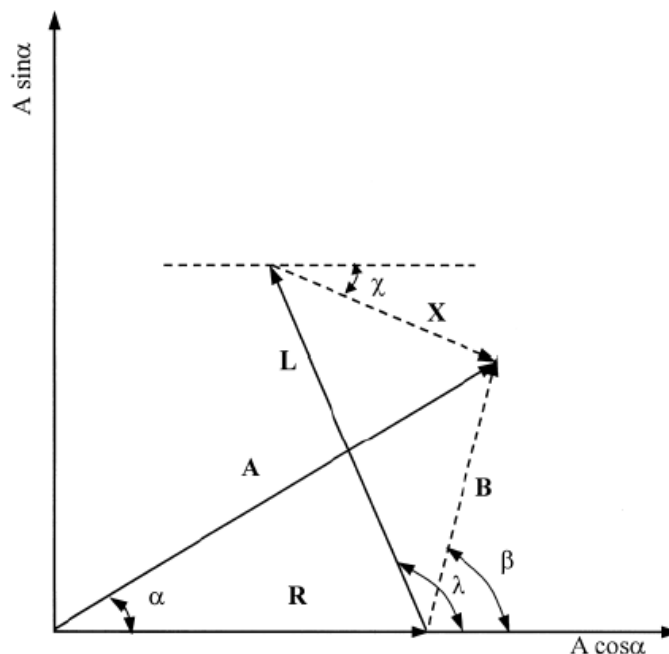
Fig. 2.1.4: For a given tidal frequency, phasor plot showing the relationship between the observed tidal amplitude vector A(A, \alpha) , the Earth model R(R, 0) , the computed ocean tides load vector L(L, \lambda) , the tidal residue B(B, \beta) = A - R and the corrected residue X(X, \chi) = B - L , after Ducarme et al. (2009).
