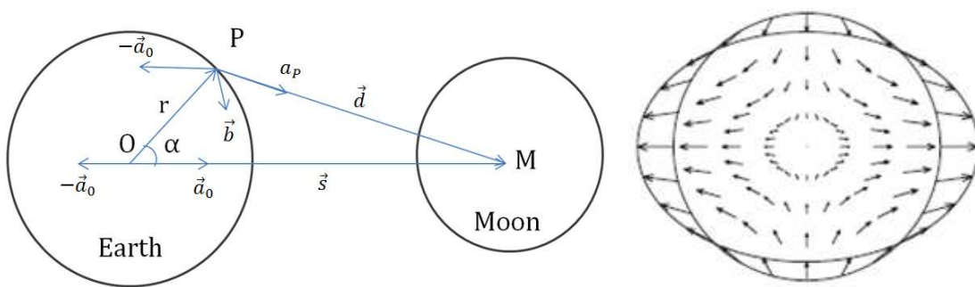
Fig. 2.1.2: Tidal forcing. The left plot shows the geometry of the problem for computing the tidal force at a point P on the Earth, given an external body M (Moon). The right plot shows the field of forces (accelerations) for the actual Earth–Moon separation. The elliptical line shows the equipotential surface under tidal forcing, greatly exaggerated (adapted from Agnew, 2007).
