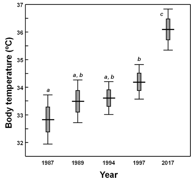
FIGURE 1 Mean values (with standard errors and 95% confidence intervals) for body (cloacal) temperatures of active lizards recorded in the same open forest ('Montes de El Pardo y Viñuelas') during the summers of different sampling years between 1987 and 2017. Letters indicate homogeneous groups according to the results of a Newman–Keuls post-hoc test following one-way ANOVA.
