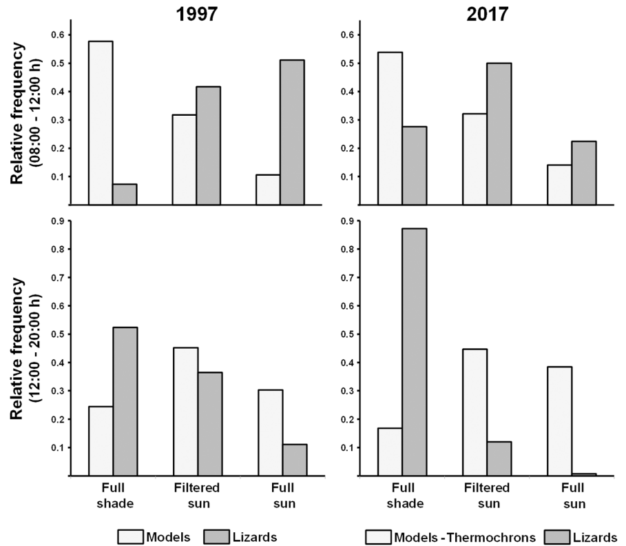
FIGURE 3 Use (lizards) and availability (models) of patches in full sun, filtered sun or full shade as a function of time interval (before vs. after 12:00h) in 1997 and 2017. Sample sizes in 1997 before 12:00h: 96 (lizards) and 359 (models); in 1997 after 12:00h: 189 (lizards) and 617 (models); in 2017 before 12:00h: 58 (lizards) and 327 (models-thermochrons); in 2017 after 12:00h: 133 (lizards) and 624 (models-thermochrons).
