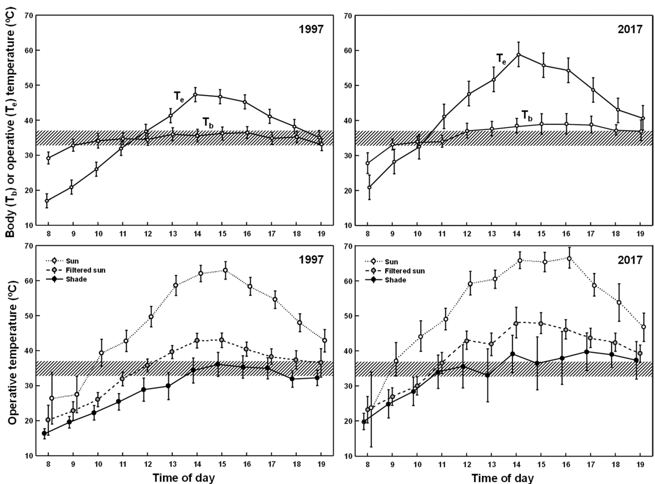
FIGURE 2 Mean values (with 95% confidence intervals) for body (cloacal) temperatures ( T_b s) and environmental operative temperatures ( T_e s) as a function of time of day in 1997 and 2017. The upper panels show the mean T_b s of active lizards and the overall means of available T_e s. The lower panels show the mean T_e s available for full sun, filtered sun and full shade locations. The selected temperature range ( T_{sel} ) is represented by the dashed areas.
