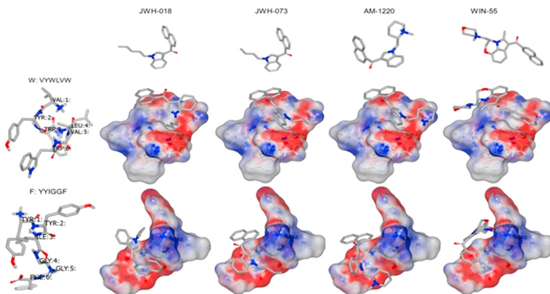
Fig. 2. Three-dimensional structures of the two hexapeptides and the 4 synthetic cannabinoids used in this work, as well as the best association complexes formed between them.
