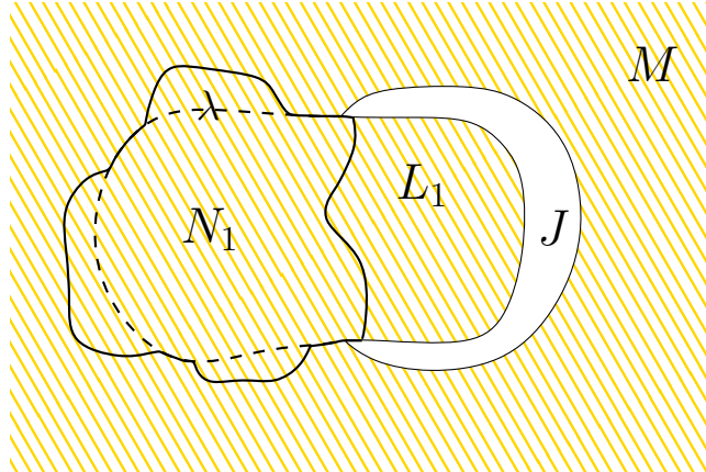
Figure 2.8: Step 2 of Lemma 2.4.9. N_0 is marked by a dashed line.
