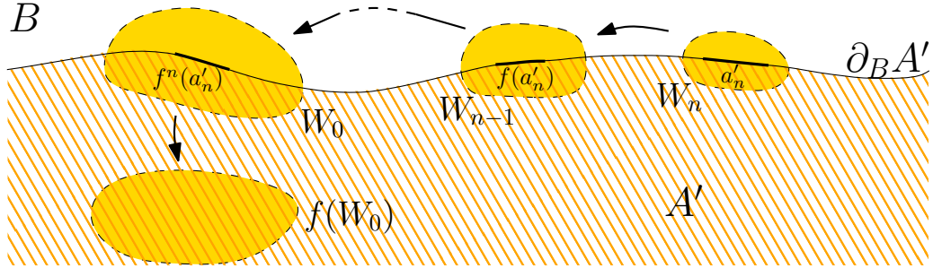
Figure 2.7: Proof of Lemma 2.4.6.
