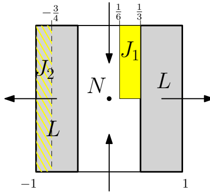
Figure 2.6: weak index pairs, Mrozek index pairs and filtration pairs are different.
