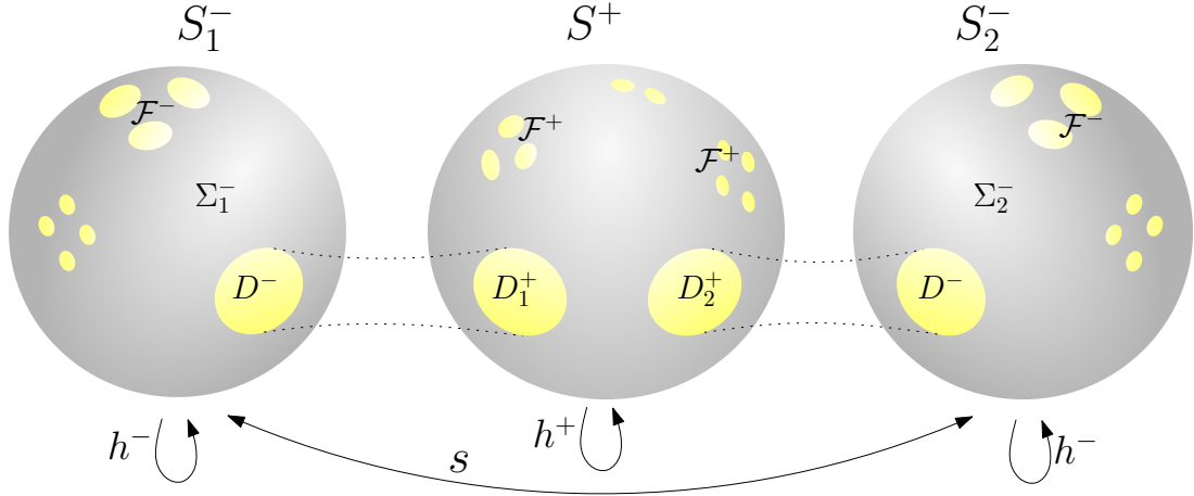
Figure 2.12: Proof of sufficiency of Theorem 2.1.8.
