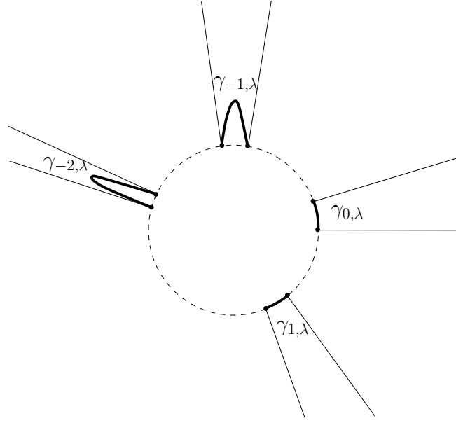
Figure 1.7: Arcs \gamma_{n,\lambda} .
