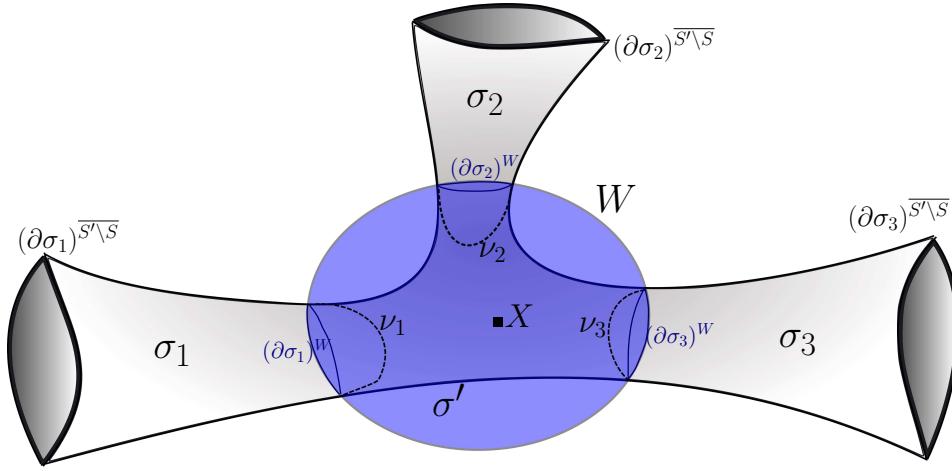
Figure 2.13: Decomposition of \sigma .
