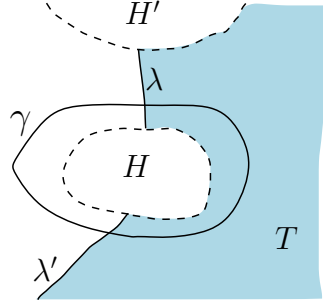
Figure 2.4: Proof of Lemma 2.3.6.
