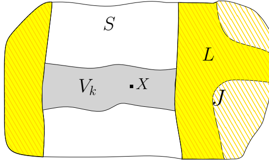
Figure 2.9: Elements of N in Lemma 2.4.18.
