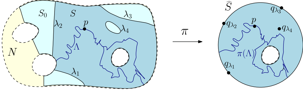
Figure 2.5: Proof of Theorem 2.3.1.
