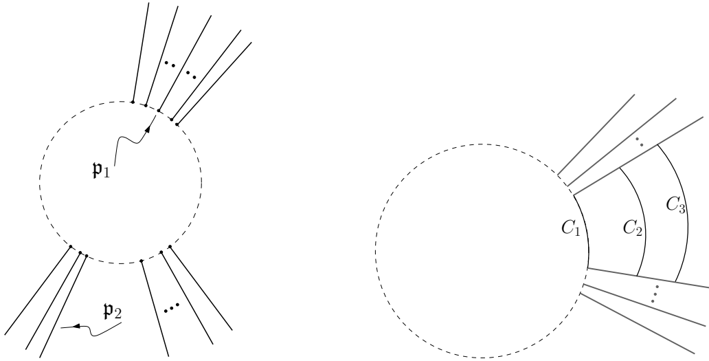
Figure 1.5: Description of the prime ends of U .
