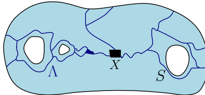
Figure 2.3: Proof of Lemma 2.3.5: All 4 (3 bounded and 1 unbounded) holes of S are separated by \Lambda .
