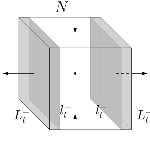
Figure 2.2: Example 2.2.18 with k = 1 and d = 3 .
