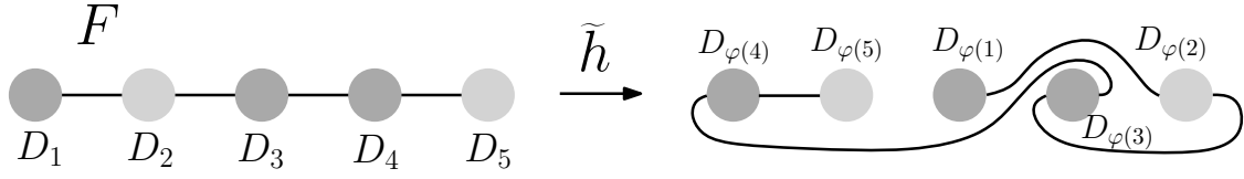
Figure 2.11: Proof of Lemma 2.5.2: example of F and \tilde{h} for \varphi : \{1, 2, 3, 4, 5\} \rightarrow \{3, 5, 4, 1, 2\} .
