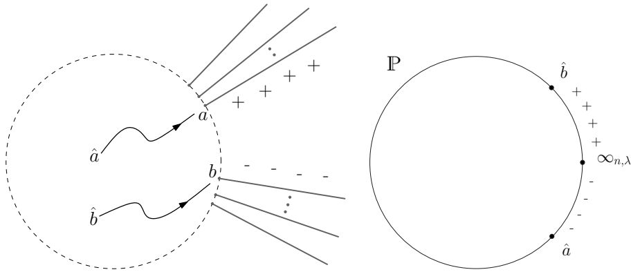
Figure 1.6: Prime ends \hat{a}, \hat{b} and \infty_{n,\lambda} .
