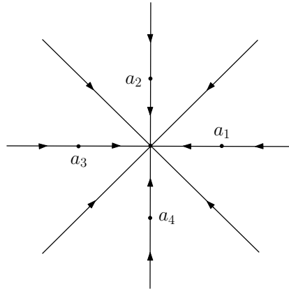
Figure 1.3: Flow \{\phi_t\}_{t \in \mathbb{R}} .
