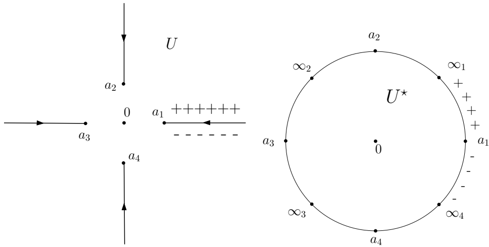
Figure 1.4: Region U (left) and its prime end compactification U^* (right).
