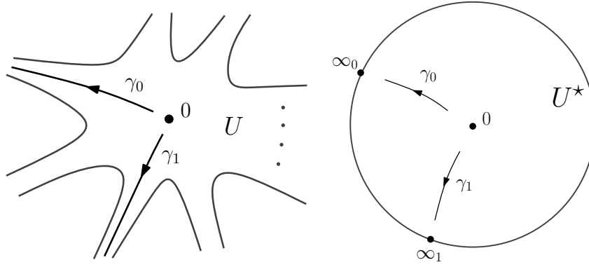
Figure 1.10: New arcs \gamma_0, \gamma_1 constructed in Step 1 .
