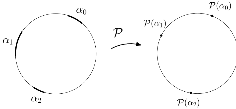
Figure 1.1: Example of Cantor function.
