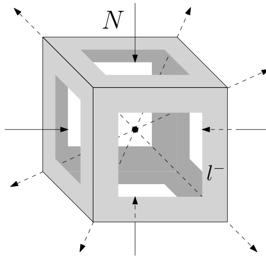
Figure 2.10: Example 2.4.24: l^- is a neighborhood of the edges of the cube N .
