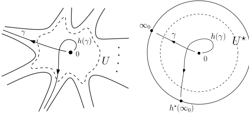
Figure 1.9: Arcs \gamma, h(\gamma) in U .
