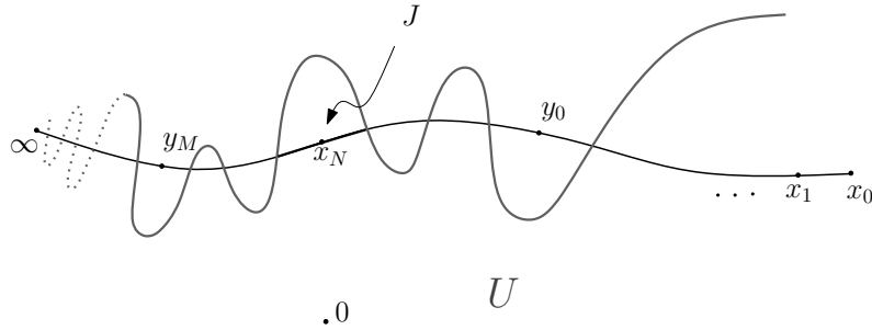
Figure 1.8: Arc \Gamma in Step 1.
