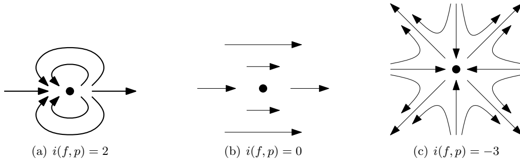
Figure 2.1: Fixed points of planar homeomorphisms.
