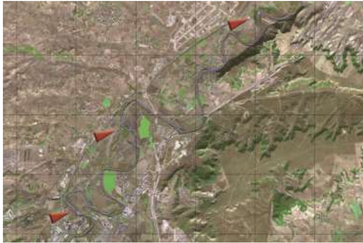
Fig. 5.5. Lower Pisuerga River, upstream Valladolid city. The arrows show the position of three weirs associated to three consecutive SHP. The length of affected stretch is 22.7 km and the medium slope is 0.03 %. The pool-riffle sequence has totally disappeared causing remarkable habitat loss and nutrient retention. As a result, the stretch becomes eutrophic in summer and the ecological regime has shifted from lotic to lentic (Ballarin & Rodriguez, 2013). Source: Iberpix. Instituto Geográfico Nacional, IGN. Grid scale: 2.5 X 2.5 Km.
