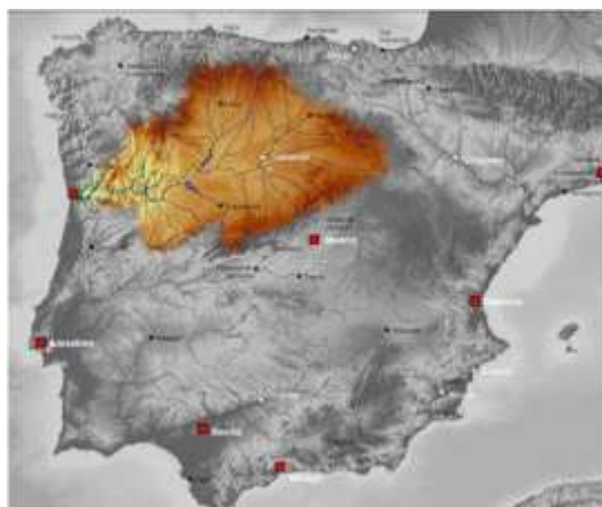
Fig. 4.1. Location of the Duero River Basin in the Iberian Peninsula. Source: Wikimedia Commons.
