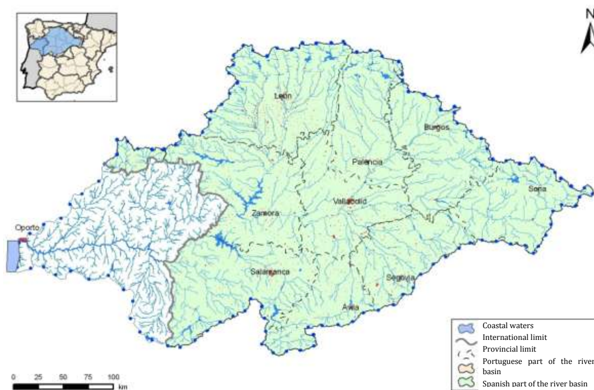
Fig. 5.2. Location of the Duero River Basin in the Iberian Peninsula. Source: OPH-CHD
