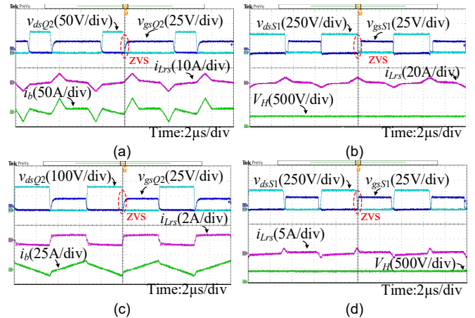
Fig. 17. ZVS experimental waveforms of switches with light load. (a) Q_2 when V_L = 18 V. (b) S_1 when V_L = 18 V. (c) Q_2 when V_L = 36 V. (d) S_1 when V_L = 36 V.
