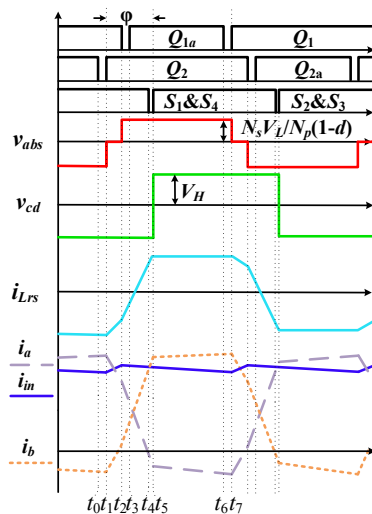
Fig. 2. Steady-state waveforms for proposed TWCI DAB in boost mode. (Interval A: \varphi \in [(2d-1)\pi, \pi] ).
