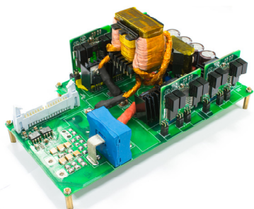
Fig.15. The experimental prototype.
