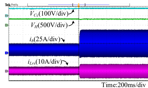
Fig. 19. Load-step experimental result from half load to full load with V_L = 27 V.
