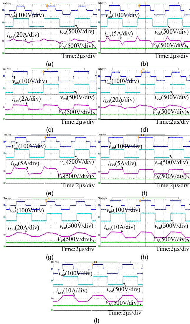
Fig. 16. Steady-state waveforms with the proposed TWCI DAB. (a) at light load when V_L = 18 V. (b) at light load when V_L = 27 V. (c) at light load when V_L = 36 V. (d) at half load when V_L = 18 V. (e) at half load when V_L = 27 V. (f) at half load when V_L = 36 V. (g) at full load when V_L = 18 V. (h) at full load when V_L = 27 V. (i) at full load when V_L = 36 V.
