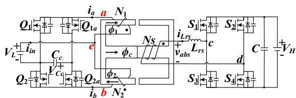
Fig. 1. The topology of proposed TWCI DAB.
