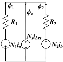
Fig. 3. Magnetic reluctance model of TWCI.
