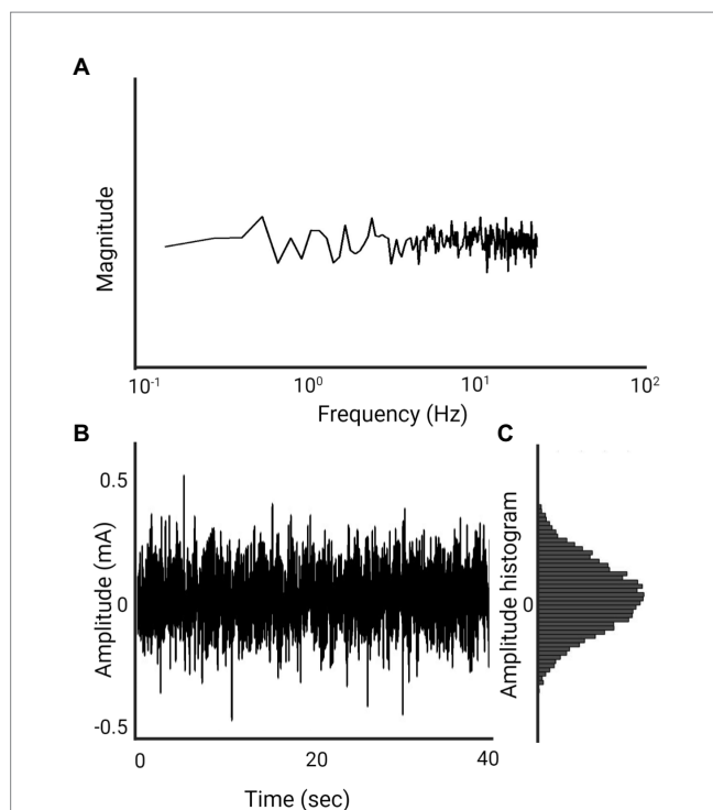
FIGURE 3 1mA, 0–30Hz Gaussian white noise nGVS signal (Created with BioRender.com). (A) Spectral frequency graph, the waveform contains frequencies between 0 and 30Hz with equal intensity at each frequency. (B) Time plot of the signal. The amplitude of 1mA means that 99% of all generated amplitude values are between 0.5mA and –0.5mA. (C) A histogram of the distribution of the signal amplitude. A random level of current generated for every sample is normally distributed, thus the probability density function follows a bell-shaped curve.
