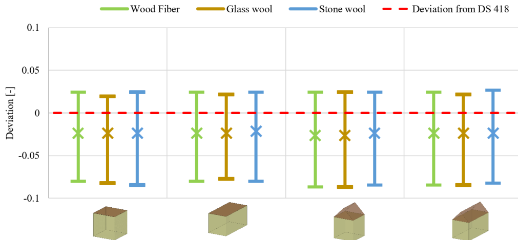
Figure 4. Difference between BSim and DS 418 calculation for different insulation materials and simplified single-zone cases, see the indication below the figure. The dotted red line indicates perfect correspondence between BSim and the DS 418 calculation, the crosses indicate the mean value and the bars indicate the minimum and maximum values. The variation is caused by solar absorptance and variation in external thermal resistance.
