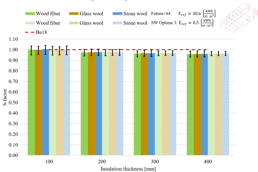
Figure 5. The ratio of transmission loss from September to April between dynamic and steady-state calculation. The fully colored bars consists of models with the window Futura+44, and the checkered bars consists of models with the window SW Optima 3. The dispersion is caused by solar absorptance, orientation of the house and the variation in external thermal resistance.
