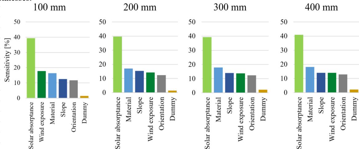
Figure 6. The sensitivity of the input parameters with respect to the transmission loss for elements with the indicated thickness of insulation. The dummy variable constitute a variable with random noise that does not influence the model, and is used as a benchmark for insignificance.
