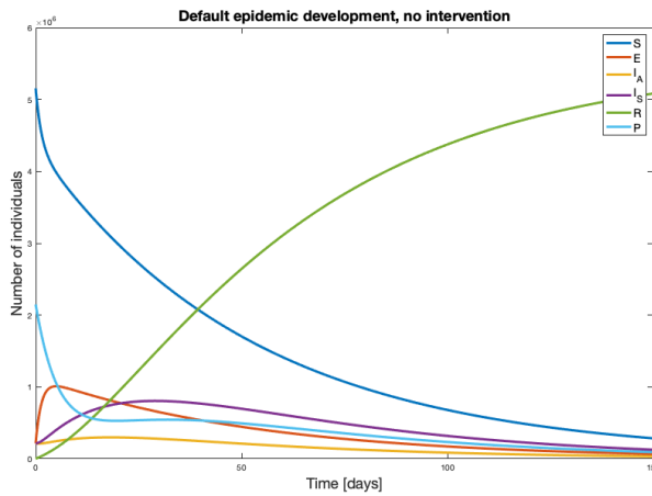
Figure 4 Simulation of epidemic development assuming no interventions. The six curves illustrate the number of: Susceptible ( S ), Exposed ( E ), Asymptomatic Infectious ( I_A ), Symptomatic Infections ( I_S ), Recovered ( R ), and Pathogens ( P ), respectively.
