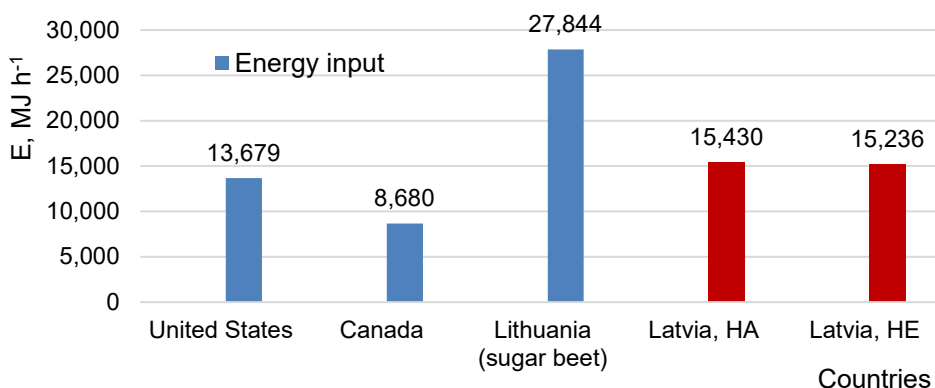
Figure 3. Comparison of energy input with the indicators of other countries (Amenumey & Capel, 2014; Bandekar et al., 2022; Bruciene et al., 2021).
