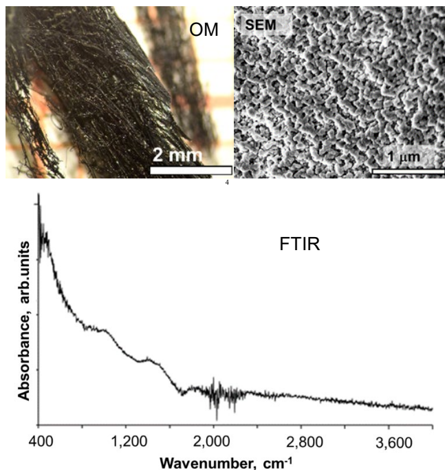
Figure 6. Surface morphology (OM), and microscale morphology (SEM) and chemical bonds (FTIR) of activated carbon from thermally treated sheep wool.
