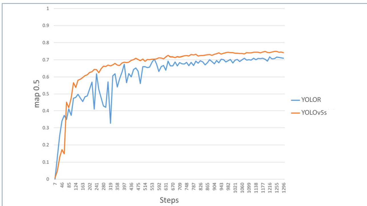
Fig. 9 mAP_0.5 comparison between YOLOv5s and YOLOR
