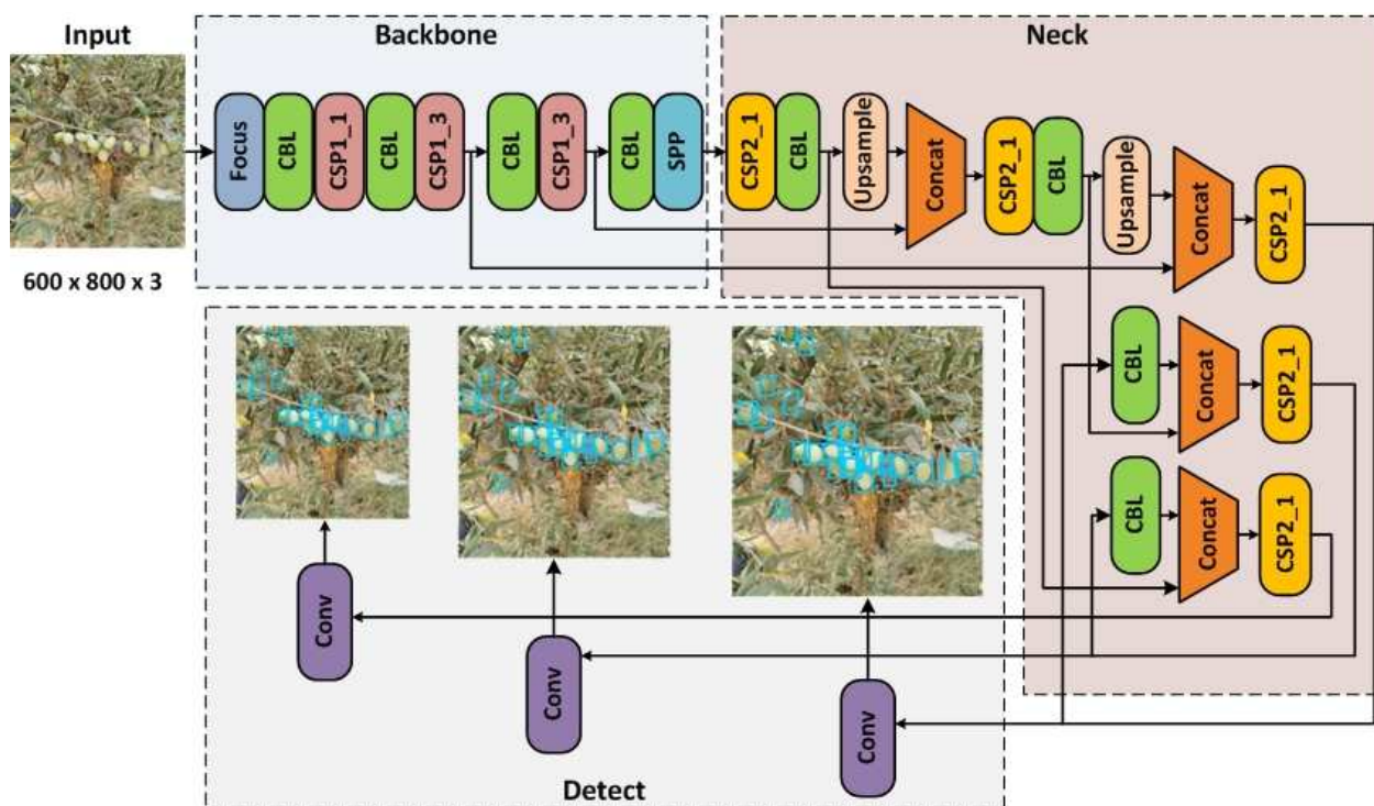
Fig. 4 YOLOv5s architecture CSP – cross stage partial network; CBL – convolution-batch normalization – leak ReLU; SPP – spatial pyramid pooling; Concat – concatenation function; Conv – convolutional layer
