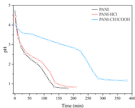
Figure 1. The changes of pH of the reaction mixture during time for PANI/ graphene composites.
