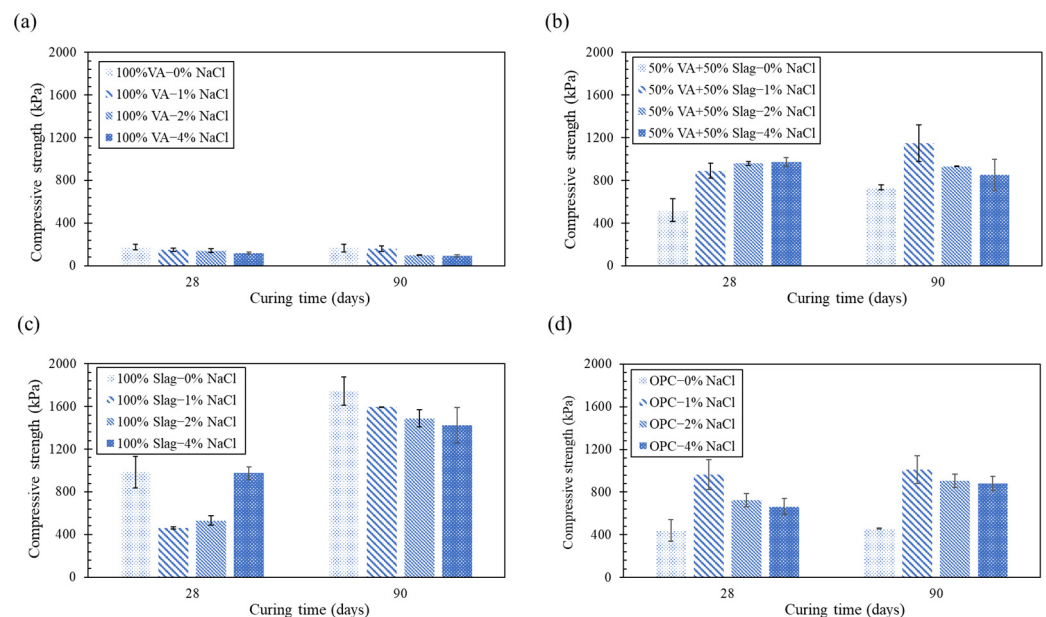
Figure 7. Effect of NaCl content and curing time on the mechanical properties of (a) alkali-activated volcanic ash, (b) alkali-activated volcanic ash and slag, (c) alkali-activated slag, and (d) Portland-cement-stabilized saline sandy soils at SC condition.
