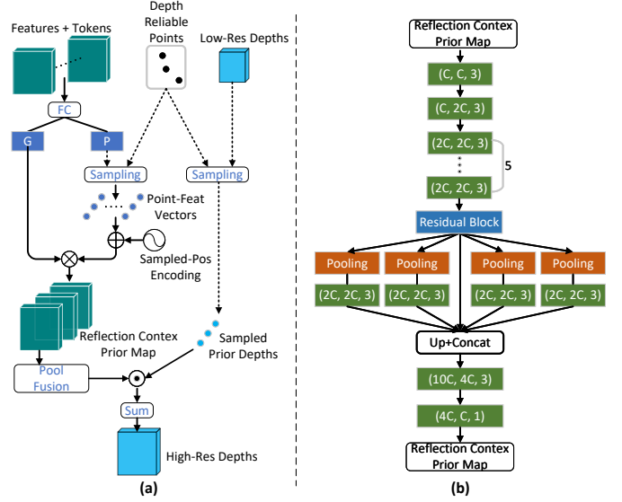
Fig. 13: (a) Reflection context guided depth estimation architecture, with \odot representing element-wise product. (b) Pooling-based convolution fusion model diagram (‘‘Pool Fusion’’ in (a)). Green rectangles labeled (C_1, C_2, K) represent convolution layers with input channel C_1 , output channel C_2 , and kernel size K . ‘‘Up’’ denotes bilinear upsampling.
