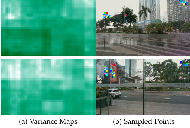
Fig. 11: Two visualized variance maps and sampled depth reliable points. The variance maps are calculated between depth estimations at 1/32 and 1/16 input resolutions. The ‘‘Sampled Points’’ are the points with top 30 values in corresponding variance maps.
