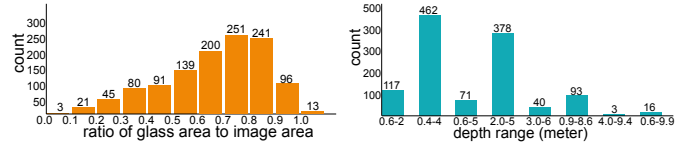
(a) Glass Area Distribution (b) Glass Depth Distribution
