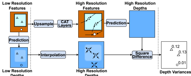
Fig. 12: Diagram for the generation of depth variance. Small triangles and circles in feature maps represent pixels in glass areas (light green) and non-glass opaque areas (brown). ‘‘CAT Layers’’ denotes class attention transformer layers.
