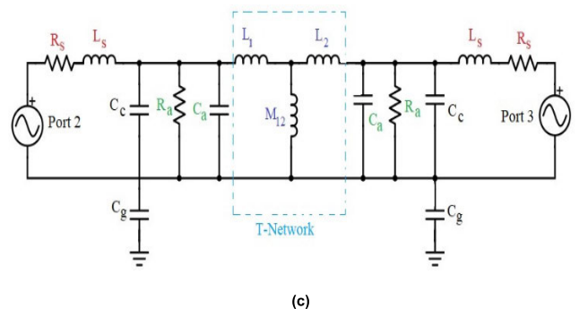
FIGURE 6. Equivalent circuit of two adjacent antenna elements: Ant 2 and Ant 3 are considered. (a) Scattering parameters of both circuit and 3D models. (b) Two individual antennas circuits coupled through a mutual inductance, M_{12} = 0.072 nH. (c) Over all equivalent circuit model of Ant 2 and Ant 3, M_{12} = 0.072 nH, L_1 = L_2 = 1.23 nH.
