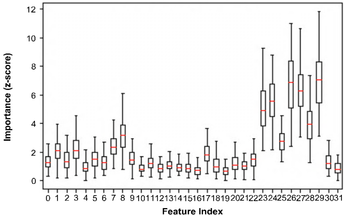
Figure 20: Feature importance in terms of z\text{-score} distributions of RF permutations for the highly important feature subset nominated by Boruta.
