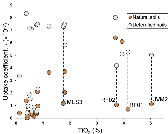
Fig. 5. Photocatalytic efficiency as a function of TiO 2 . Red soils, rich in hematite (MES3, RF02, RF01 and JVM2) increase their photocatalytic efficiency (uptake coefficient) once their iron oxide pigments were selectively removed (grey) from the natural soil (orange). A small Ti oxide content of <1%, is enough to achieve a high photocatalytic efficiency.
