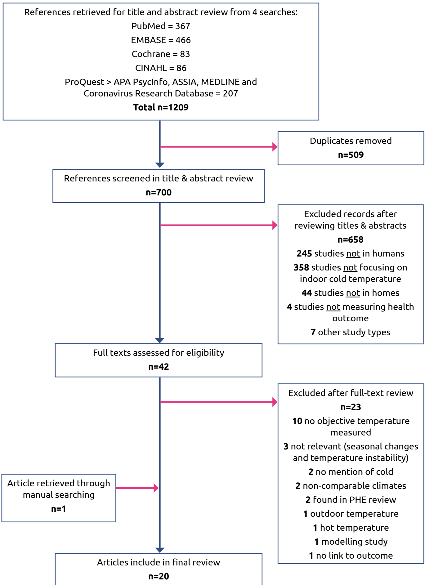
Figure 3. Search process
