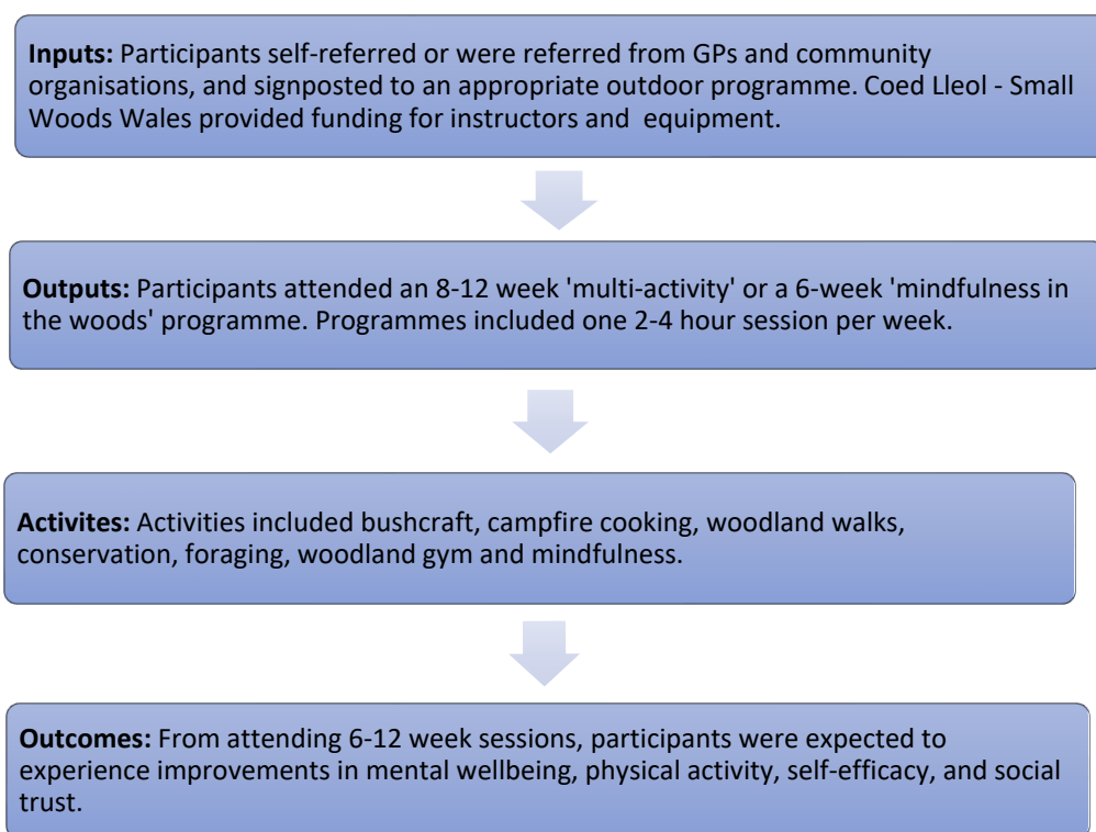
Figure 2. Logic Model.
