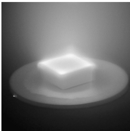
Image of a diamond single crystal during growth by plasma-assisted chemical vapour deposition. Image credit: Laboratoire des sciences des procédés et des matériaux, Villetaneuse, France.
