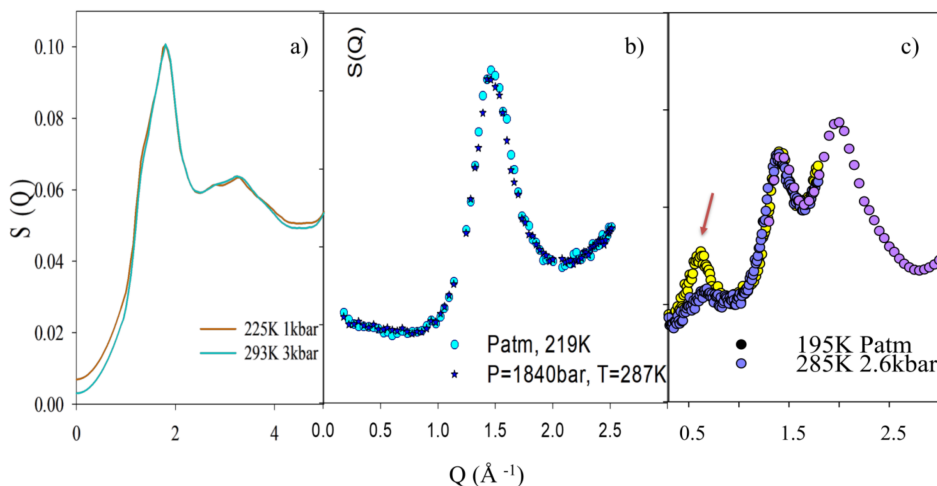
Figure 4. Static Structure factor along an isochore, T and P are indicated in the plot: a) a van der Waals liquid, toluene \rho = 1.06\text{g}/\text{cm}^3 ; b) a polymer, polubutadiene, M_w=7000 , \rho = 0.94\text{g}/\text{cm}^3 ; c) an hydrogen bonded liquid m-fluoroaniline \rho = 1.3\text{g}/\text{cm}^3 , here the arrow indicates the position of a prepeak due to the presence of H-bond induced clusters and its T-dependence associated this the strength of the H-bond [75].
