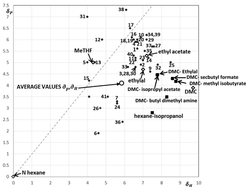
Fig. 4. Hansen parameters for studied solvents, new alternative solvents as pure components and binary azeotropic mixtures.
