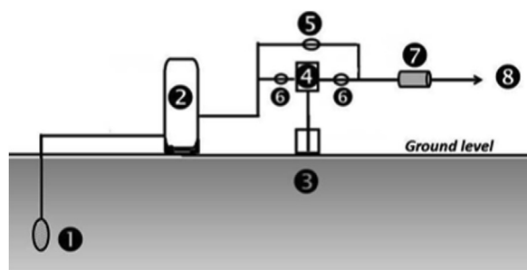
Fig. 1. Schematic view of the farm's water distribution system. 1: Borehole pump, 2: water buffering tank, 3: Dinastim™ or Pigfast™ delivery tank, 4: dosing distribution pump, 5: bypass, 6: pumps, 7: position of experimental coupons, and 8: to the troughs.
