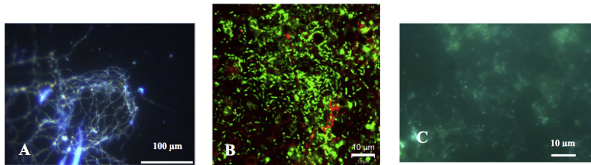
Fig. 3. Observations in confocal microscopy of the water pipe's inner surface (Breeding Unit A). A, T 0 , B, T 8 , C, and T 13 . A and C are labelled with DAPI, B is labelled with the Dead/Live kit so that living cells exhibit green fluorescence whereas dead ones appear red.
