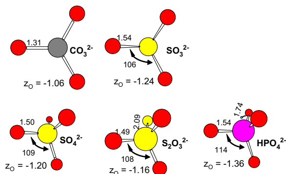
Fig. 5. Geometry of RO 2 - ligands optimized in the gas phase. R–O bond distances (Å), angles (°) and z O , the atomic charge of O are written on the figure.
