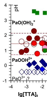
Fig. 8. Predominance diagram of Pa(V) hydrolysis species. The hydrolysis constants ( -\log^* K_i^\circ = \text{pH}_{1/2,i} correspond to the pH value at the half-point reaction) have been re-interpreted (Table 3) from the experimental data (and extrapolated to I = 0 with the SIT formula) of Ref. [30] in 0.1 (open symbols) to 3 (filled symbols of the same colour) \text{mol L}^{-1} \text{NaClO}_4 aqueous solutions for the successive formations of species of charges 2 (dark blue diamonds), 1 (brown circles) and 0 (green squares). The intermediate colours are for 1 and 0.5 \text{mol L}^{-1} . For higher [\text{TTA}]_t values (not represented), a systematic deviation is observed. (For interpretation of the references to colour in this figure legend, the reader is referred to the web version of this article.)
