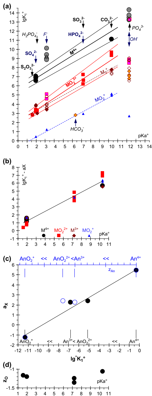
Fig. 4. Proton and other cation affinities for ligands. K_1^\circ is the standard formation constant of the \text{ML}^{2\text{M}+2\text{L}} complex, and K_a^\circ is the protonation constant of the \text{L}^{2-} ligand written on the figure (Table 1). Since all the (\log K_{1,X}^\circ = a_X + b_X \text{p}K_a^\circ) lines are virtually parallel for all the (X) oxidation states (a). We also used the same ( b_X = 0.62 \pm 0.16 ) slope in \log K_{1,X}^\circ - a_X = ((0.62 \pm 0.16) \text{p}K_a^\circ) regressions for the \text{RO}_2^{2-} ligands, and shifted the curves by a_X (b): a_X - a_{\text{VI}} = (\log K_{1,X}^\circ - \log K_{1,\text{VI}}^\circ) = \log K_{X/\text{VI}}^\circ (Eq. (5)), where K_{X/\text{VI}}^\circ is the constant for the \text{AnO}_2\text{RO}_2/\text{MRO}_2^{2\text{M}-2} exchange equilibrium (Eq. (6a)) for \text{M}^{2\text{M}} = \text{An}^{3+} , \text{An}^{4+} or \text{AnO}_2^{2+} . For An at the oxidation state X, a_X (= \log K_{1,X}^\circ - 0.62 \text{p}K_a^\circ) can be used as a definition of a quantitative scale for the (up to now qualitative) \text{An}^{4+} > \text{AnO}_2^{2+} \approx \text{An}^{3+} > \text{AnO}_2^+ series (y axis of (c)). It is compared (black filled symbols) with the hydrolysis constant ( K_1^\circ ) scale on the x axis (of (c)), and z_{\text{An}} , the An atomic charge (blue open symbols corresponding to the top scale). z_O , the atomic charge of O in \text{RO}_2^{2-} is not specially correlated with its \text{p}K_a^\circ (d). The x-axes are the same for (a), (b) and (d); the names of the ligands are only written on (a).
