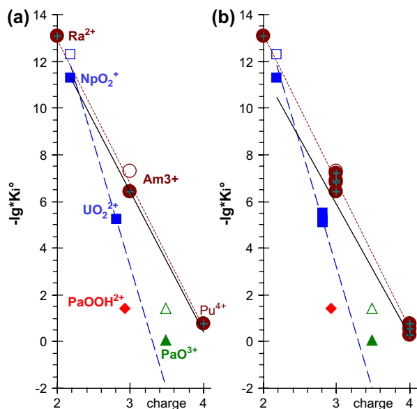
Fig. 9. Hydrolysis constants of actinide aqueous ions: -\lg^*K_1^\circ (filled symbols) and -\lg^*K_2^\circ (open symbols). The lines represent the linear regressions for (black line) all the points plotted on the figures excepted Pa(V) ones, only for the ( \text{Ra}^{2+} , \text{Am}^{3+} , \text{Pu}^{4+} ) set (brown dotted line), or only for the ( \text{NpO}_2^+ and \text{UO}_2^{2+} ) set (blue dashed line). The (atomic NPA) charges of the bare An cations (written in Fig. 9(a)) were obtained from DFT quantum calculations in gas phase. Data and corresponding lines are plotted by adding similar cations in Fig. 9(b). Two possible stoichiometries of “the” Pa(V) aqueous species are represented. (For interpretation of the references to colour in this figure legend, the reader is referred to the web version of this article.)
