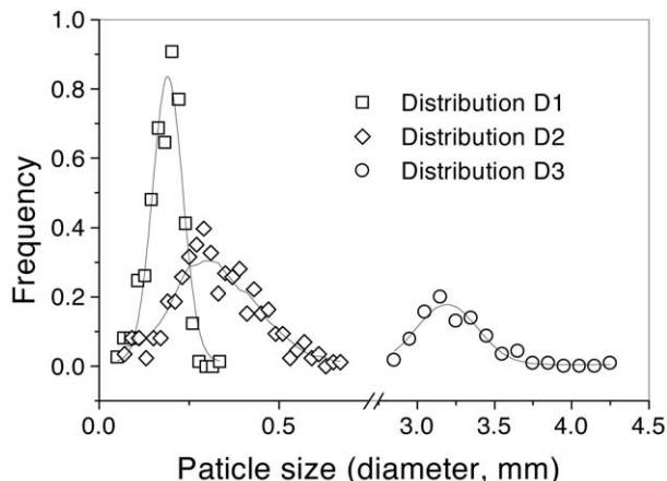
Fig. 8. Three size distributions of soda–lime–silica glass particles used in [9].
