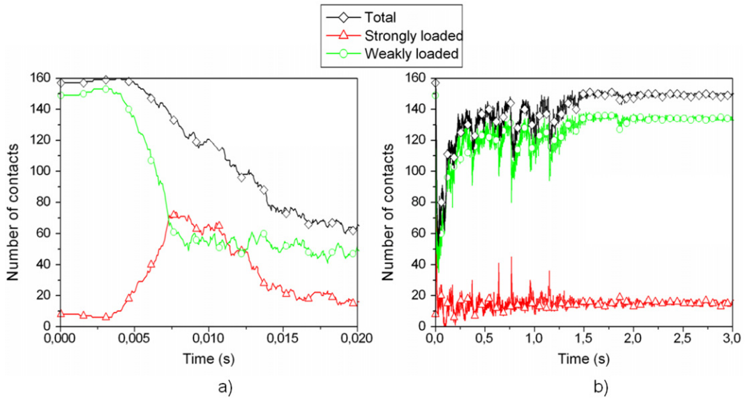
Fig. 5. Time evolution of the total number of contacts and of the number of contacts associated with, respectively, strong and weak force networks for the concentric crown located at h = 12R_m from the impact point and for both short (a) and long (b) durations.
