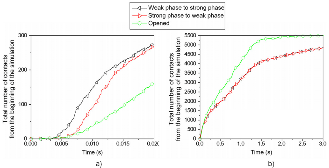
Fig. 6. Concentric crown located at h = 12R_m from the impact point: total number of contact from the beginning of the simulation which were transferred from the strong force network to the weak force network, from the weak force network to the strong force network and which were opened for short (a) and long (b) durations.
