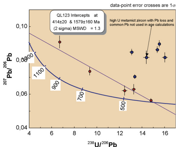
Fig. 6. Tera–Wasserburg diagram for the zircons of sample QL 123, analyzed by ICPMS.
