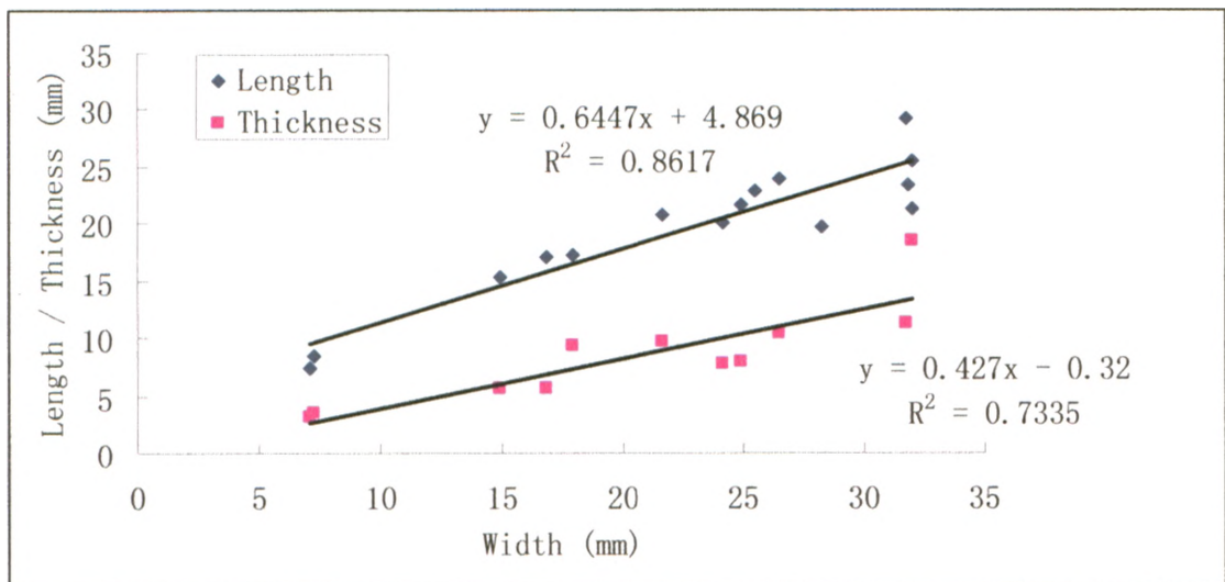
Fig. 2-18. Length-width and thickness-width graphs for complete specimens of Callipleura nobilis (Hall, 1860), sample from Collecting locality I, Coral Unit, Hungry Hollow Member, Widder Formation.
