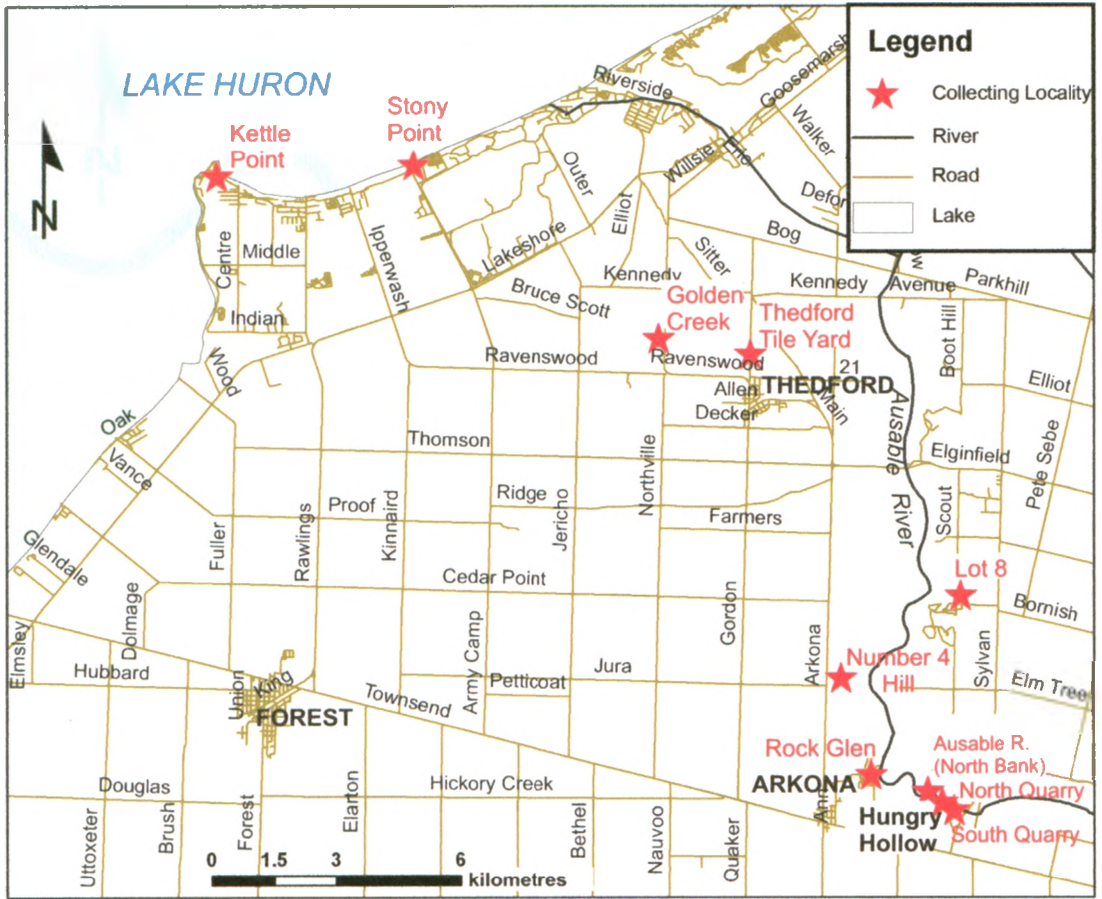
Fig. 1-5. The geographic map showing the 10 brachiopod collecting localities which have been mentioned in this thesis.
