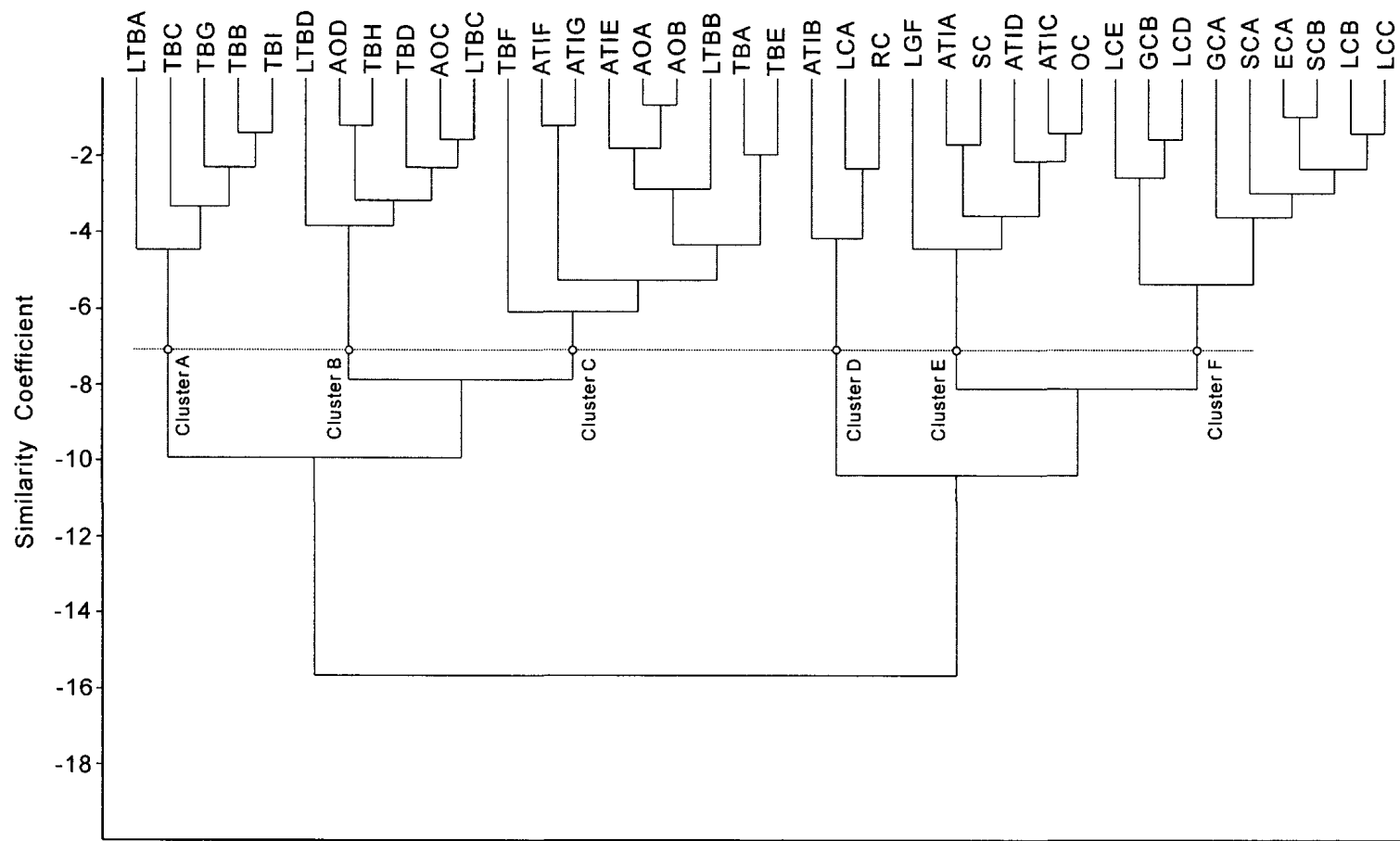
Fig. 3-2. Q-mode (taxa as variables) cluster analyses of 38 brachiopod associations from the Middle Devonian Hamilton Group of southwestern Ontario and the equivalent strata in the Appalachian Basin and the Michigan Basin, using the algorithm of Ward's method in the software package of PAST (Hammer and Harper, 2007) (See Appendix A for abbreviations of faunal occurrences).
