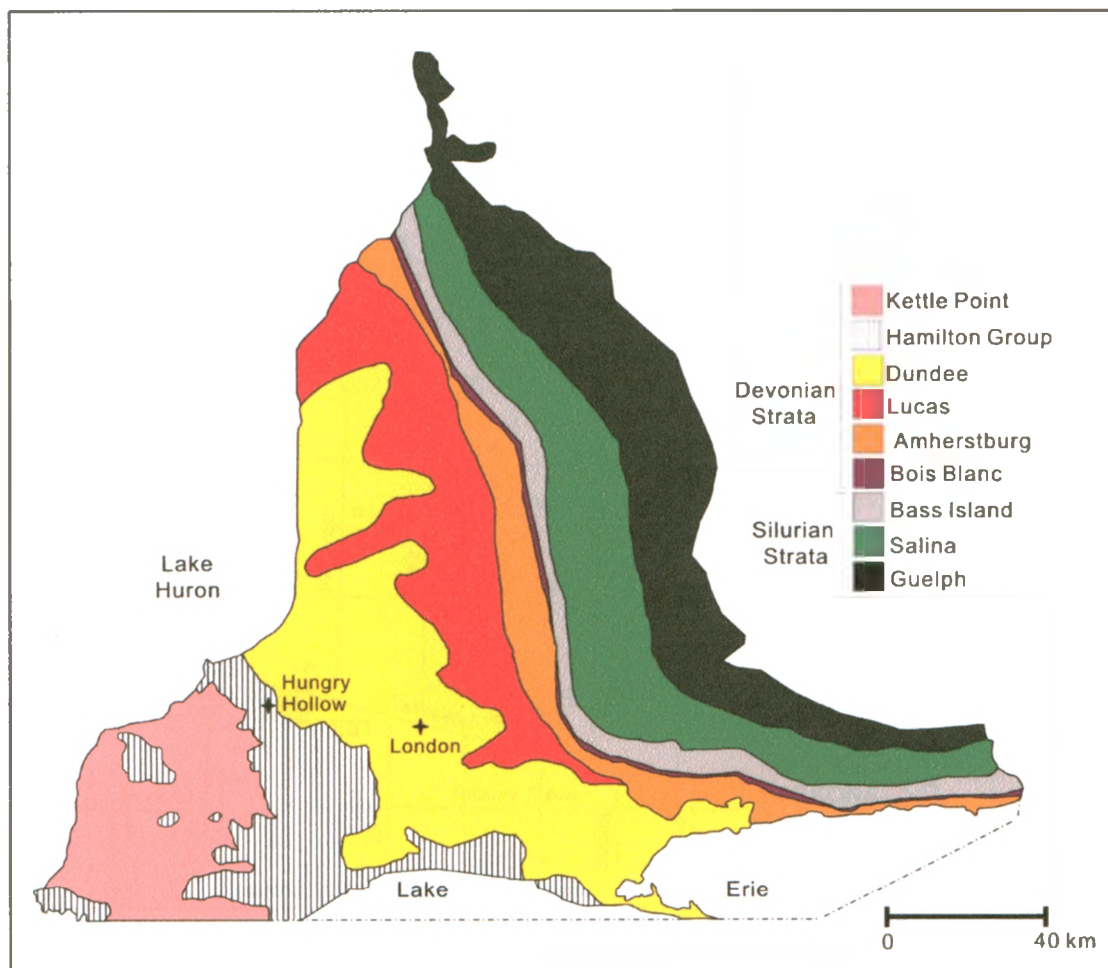
Fig. 1-4. Geological map of southwestern Ontario (After Telford, 1975).
