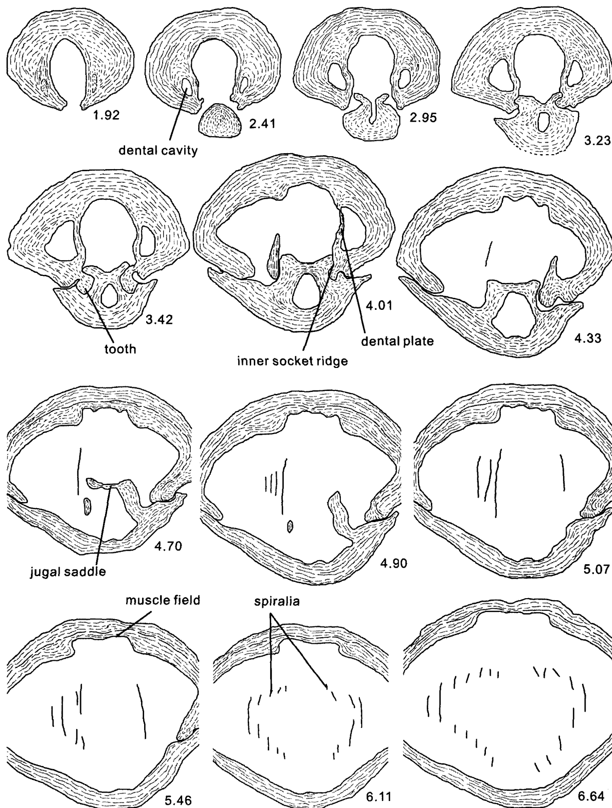
Fig. 2-29. Selected transverse serial sections of Athyris vittata Hall, 1860. W 2850. Theford Member, Widder Formation. Collecting locality 3. Distances in mm from posterior tip of ventral umbo. X4.5
