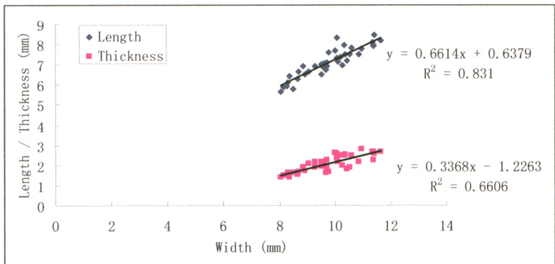
Fig. 2-7. Length-width and thickness-width graphs for complete specimens of Devonochonetes arkonensis n. sp., sample from Collecting locality I, Arkona Shale Formation.
