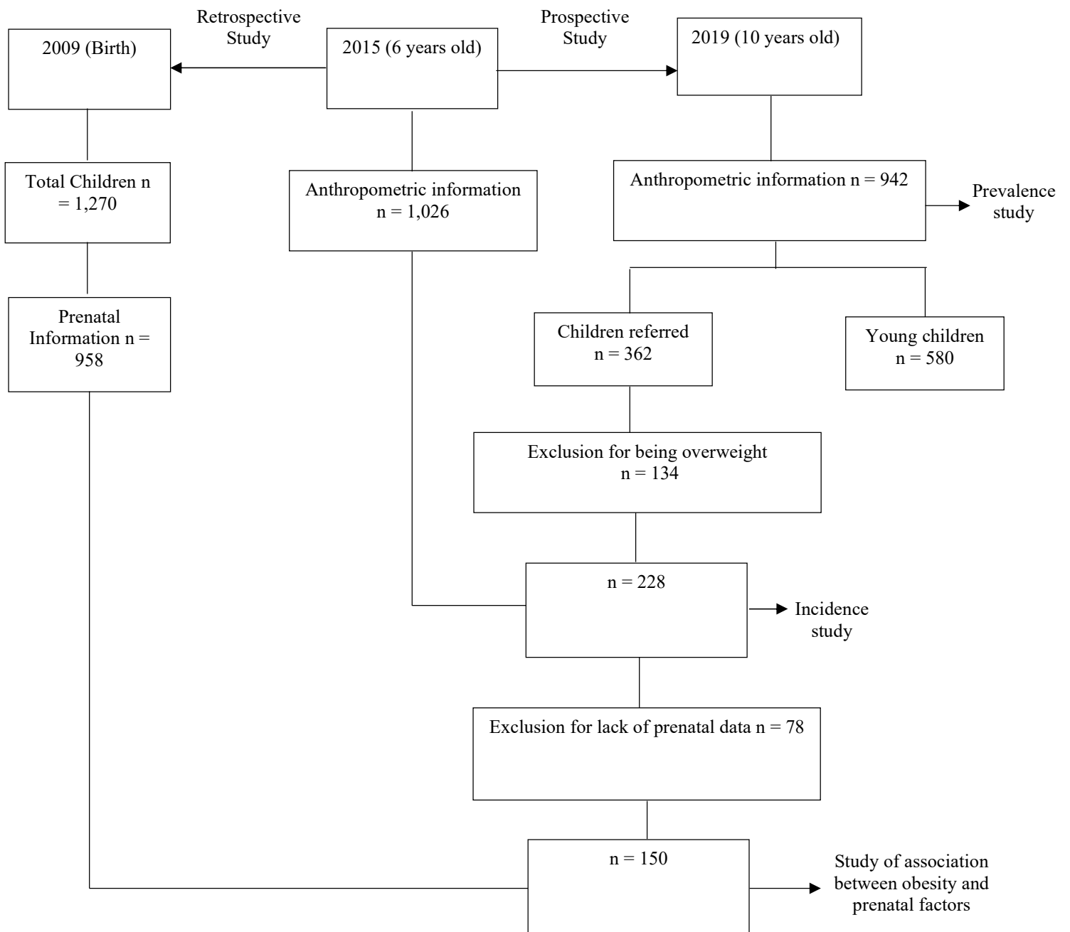
Figure 1 – Sample flowchart.
