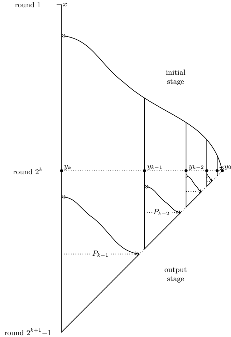
Fig. 1. Binary pebbler P_k(x) , where y_i = f^{2^k - 2^i}(x) for i = k, \dots, 0 .
