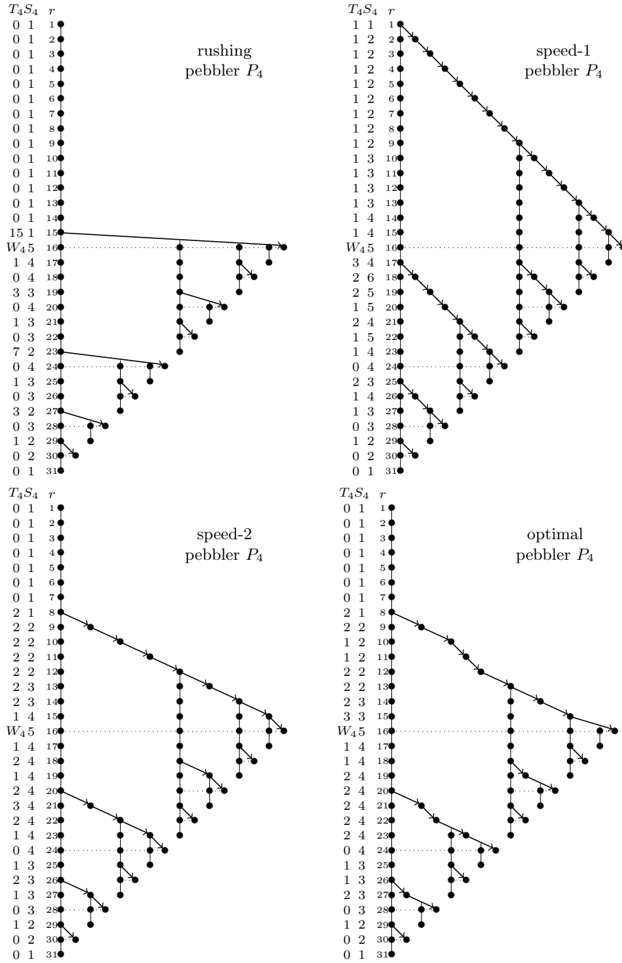
Fig. 2. Schedule T_4 , work W_4 , storage S_4 for binary pebbles P_4 in rounds 1–31. Bullets represent stored values, arrows represent hashing, vertical lines represent copying.
