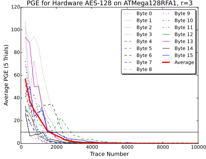
Fig. 8. Attacking intermediate rounds in the AES peripheral is also successful using the same leakage assumptions as the first-round attack.
