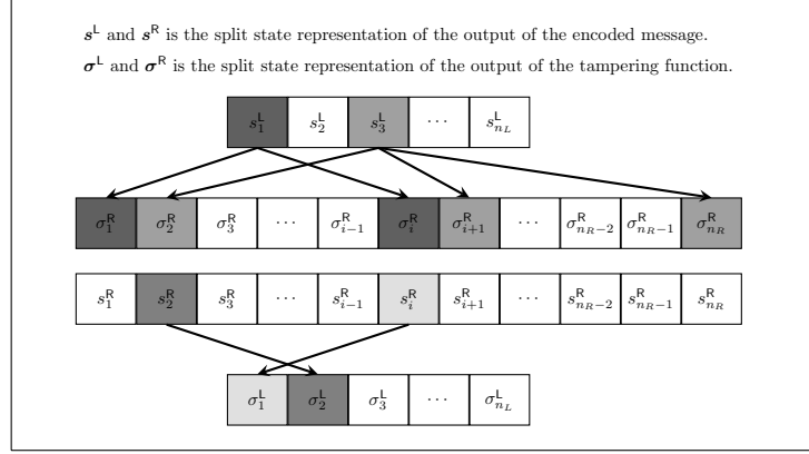
Fig. 2. The adversary chooses tampering function f = (f^L, f^R) \in \text{Local}_{\ell_i(k)}^{\ell_o(k)} which takes inputs (\mathbf{s}^L, \mathbf{s}^R) and produces outputs (\boldsymbol{\sigma}^L, \boldsymbol{\sigma}^R) . The highlighted bits of \mathbf{s}^L and \mathbf{s}^R are the “bad” bits. E.g. note that bits s_2^R and s_i^R affect the output bits \sigma_2^L and \sigma_1^L respectively after f^L is applied to (\mathbf{s}^L, \mathbf{s}^R) . Thus we add 2 and i to the set \mathcal{S}_{R \rightarrow L} . Similarly, the bits s_1^L and s_3^L affect the bits \{\sigma_1^R, \sigma_i^R\} and the bits \{\sigma_2^R, \sigma_{i+1}^R, \sigma_{n_R}^R\} respectively after the tampering function f^R is applied to (\mathbf{s}^L, \mathbf{s}^R) . We therefore add 1 to the sets \mathcal{S}_{L \rightarrow R}^1 and \mathcal{S}_{L \rightarrow R}^i , while we add 3 to the sets \mathcal{S}_{L \rightarrow R}^2, \mathcal{S}_{L \rightarrow R}^{i+1} and \mathcal{S}_{L \rightarrow R}^{n_R} . We also add both 1 and 3 to the set \mathcal{S}_{L \rightarrow R} .
