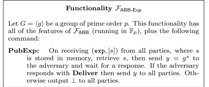
Figure 5: Ideal functionality for public exponentiation
