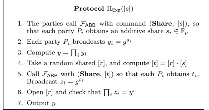
Figure 4: Securely computing a public exponentiation
