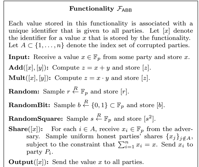
Figure 3: Ideal functionality for arithmetic MPC
