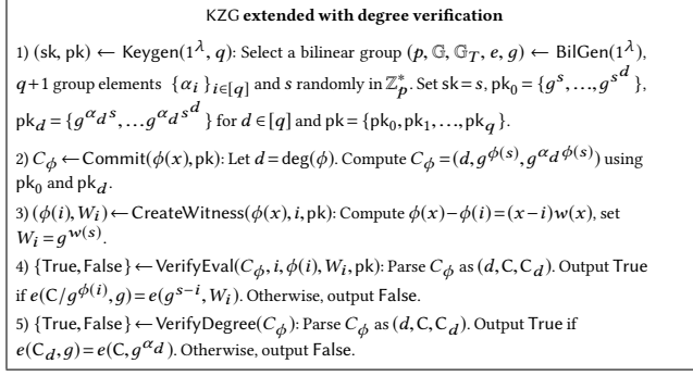
Figure 18: KZG [50] extended with degree verification.
