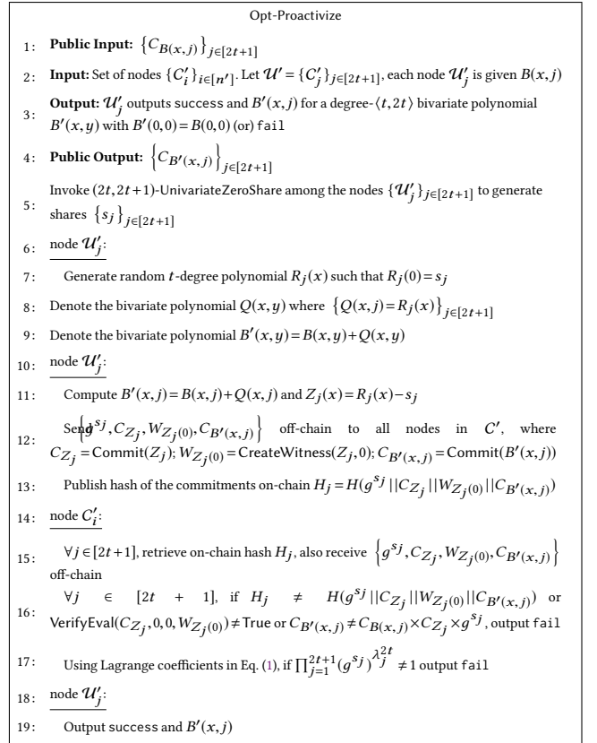
Figure 12: Opt-Proactivize updates the reduced shares.
