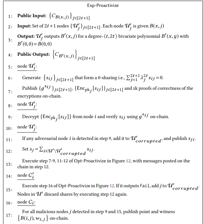
Figure 15: Exp-Proactvize protocol.
