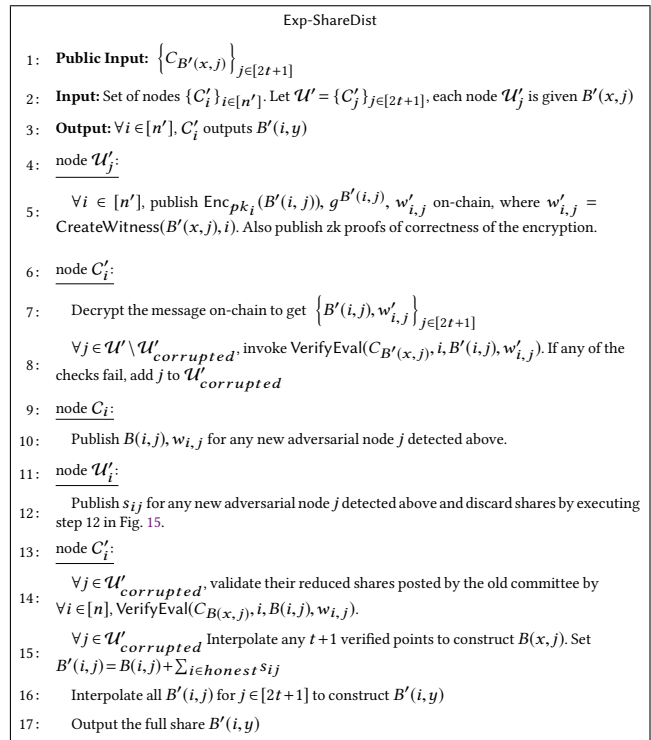
Figure 16: Exp-ShareDist protocol.
