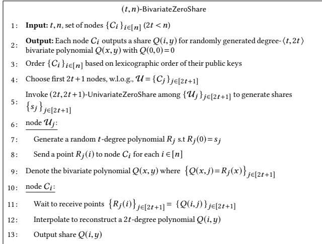
Figure 10: (t, n)-BivariateZeroShare between n nodes. A 0-hole bivariate polynomial Q of degree-(t, 2t) is generated.
