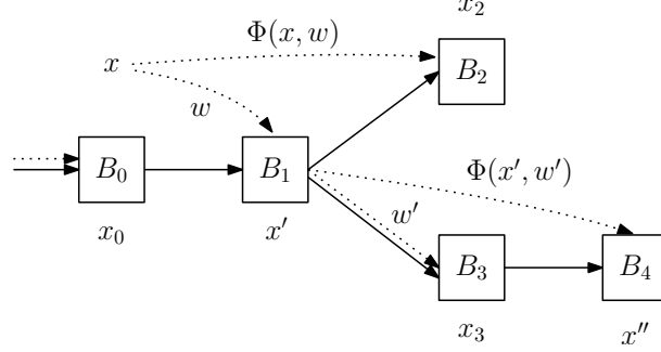
Figure 1: A possible scenario according to Lemma 21. The blocks have been generated in order B_0, B_1, B_2, B_3, B_4 , with B_3 being the only adversarial block. The cases where a valid witness is either known or can be extracted, and a NIZK proof has either been computed or simulated for the depicted transitions, correspond to the dotted and normal arrows, respectively.
