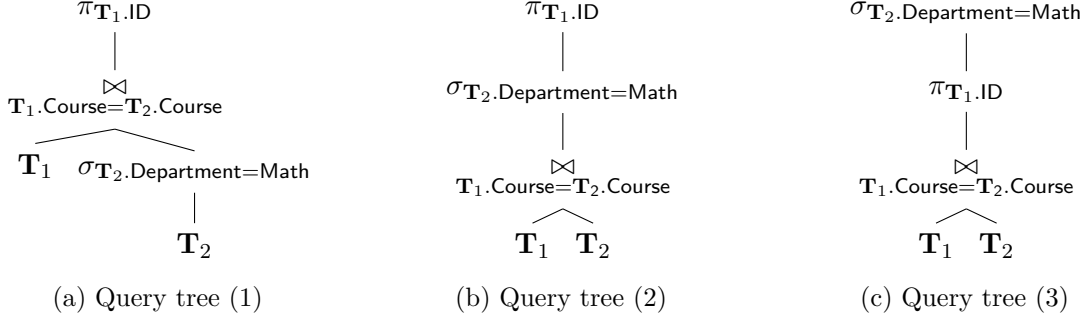
Figure 1: Different query tree representations for the same SPC query.
