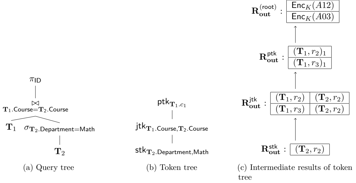
Figure 8: A query tree translated to a token tree which is then executed using the indexed database.
