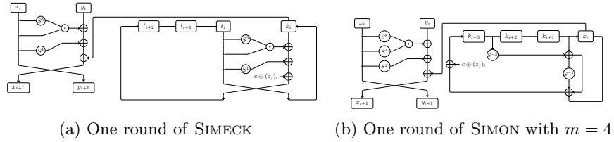
Fig. 1: Illustration of the SIMECK and SIMON ciphers
