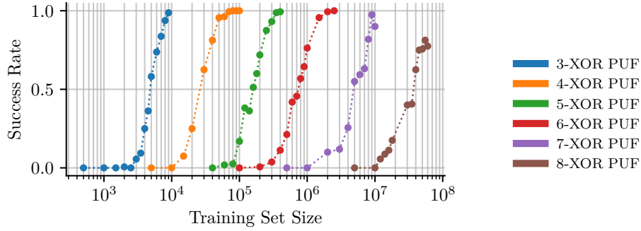
(a) LR Attack on XOR Arbiter PUF
