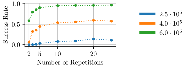
Figure 7: The impact of selecting different repetition numbers for the reliability computation on the success rate is shown for an attack on the (1,8)-iPUF. Per point, 20 PUF instances with eight trials were attacked. Each curve depicts the success rate for a different training set size.
