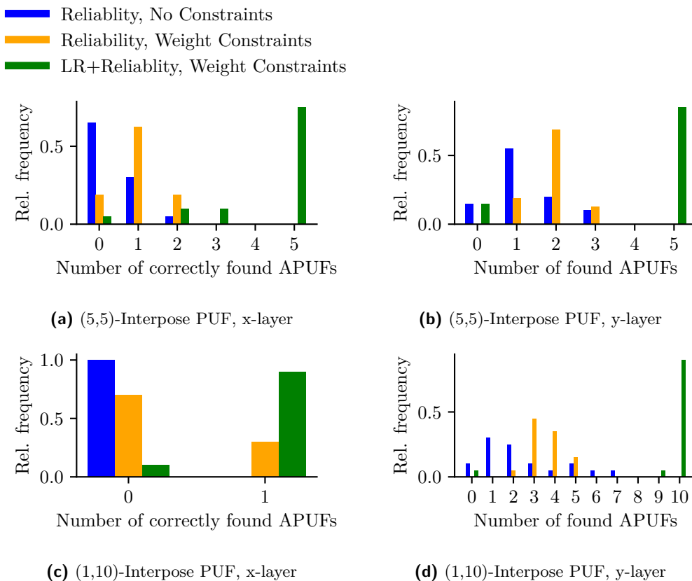
Figure 5: Result of different machine learning attacks on iPUF constructs. In each experiment, 20 PUFs were attacked with eight trials in parallel in which the best trial was chosen for the attacks with constraints and 8(x + y) trials for the unconstrained reliability attack which targets a single PUF model. An APUF is considered to be found when the Pearson correlation between PUF and model is larger than 0.99. The (5,5)-iPUF was learned with 200,000 unique challenges, (1,10) with 500,000. In both cases \sigma^2 was set to 0.1 and reliability information was collected over 10 repetitions.
