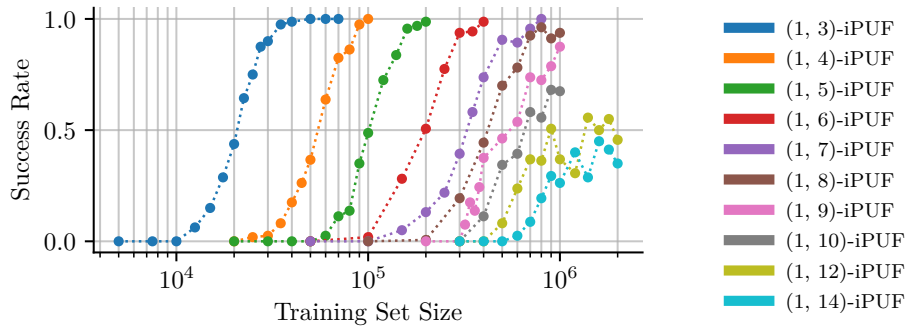
(b) Combined Reliability Attack on iPUF
