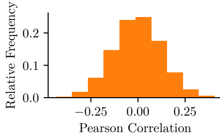
Figure 4: The distribution of the pair-wise Pearson correlation coefficient for 100 vectors of 64 i.i.d. normal distributed elements, which represent random APUF instances. The expected correlation between pairs is rather low which can be used as an argument for constraining APUF candidates in a reliability attack to have low correlation. However, the constraint should not be enforced too strictly, which would be detrimental as the true correlation has some expected deviation from zero.
