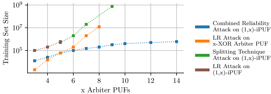
(c) Training Set Size Scaling
