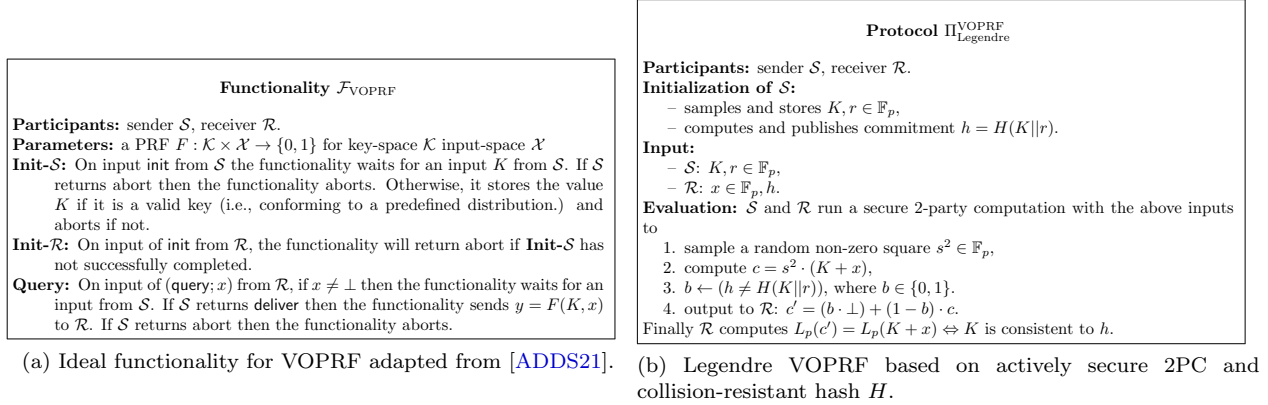
Figure 7: Legendre VOPRF.
