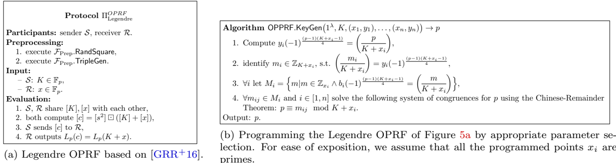
Figure 6: Legendre OPRF and the algorithm to extend it to be an OPPRF.
