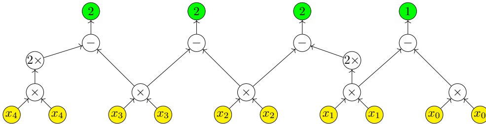
Figure 4: Arithmetic circuit representation of the ZKP statement that proves the relation \mathcal{R}_{PRF} = \{\{5\}_K = (1, 1, -1, -1, 1), K\} from Example 1 where 2 is the least quadratic non-residue. Applying our Legendre PRF arithmetization, the PRF evaluator proves that it knows the zeros of the following polynomials ( 2x_4^2 - x_3^2 = 2, x_3^2 - x_2^2 = 2, x_2^2 - x_1^2 = 2, x_1^2 - x_0^2 = 1 ). Secret input nodes are colored with yellow, while public output nodes are colored with green. Nodes with 2x denote a multiplication gate, where one of the inputs is the constant quadratic non-residue 2. Note, that for any Legendre PRF statement \mathcal{R}_{PRF}^* the arithmetic circuit has a constant multiplicative depth of two.
